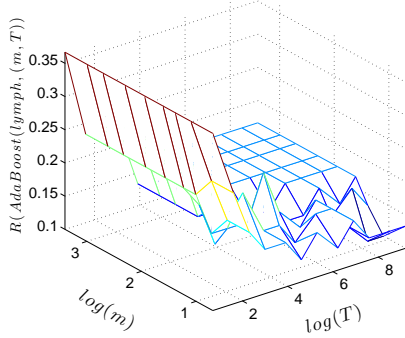
(a) Error surface of AdaBoost on lymph
