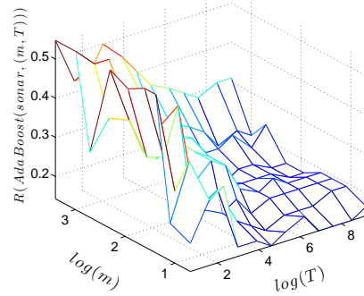
(b) Error surface of AdaBoost on sonar
