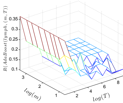
(a) Error surface of AdaBoost on lymph
