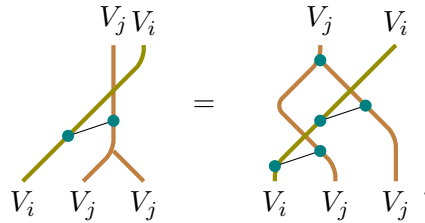
Figure 7.15: Naturality with respect to \mu_j .
