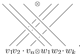
Figure 2.3: Pre-braiding extended to T(V)
