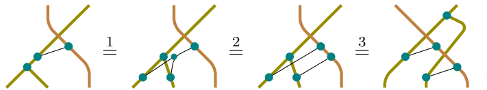
Figure 7.14: Naturality with respect to \mu_i : details
