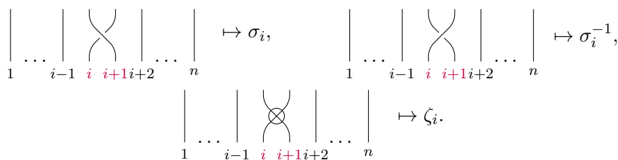
Figure 8.8: A topological version of VB_n
