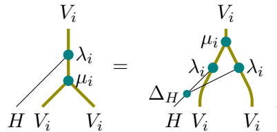
Figure 7.17: Alternative compatibility condition
