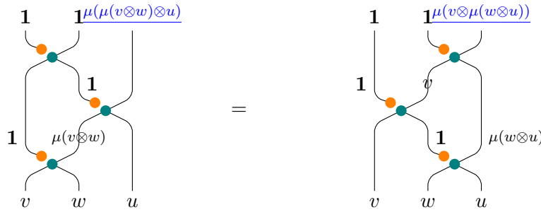
Figure 4.4: Pictorial proof of lemma 4.3.1
