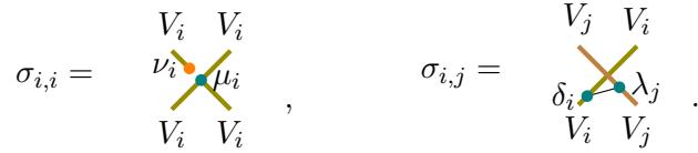
Figure 7.12: Pre-braiding for a Yetter-Drinfel'd system
