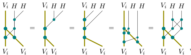
Figure 7.20: Almost a bialgebra
