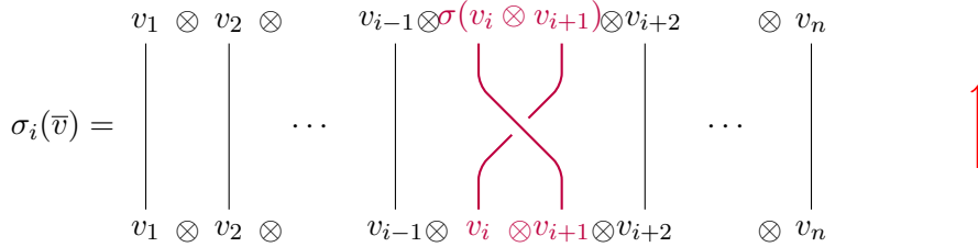
Figure 2.1: B_n^+ acts via pre-braidings
