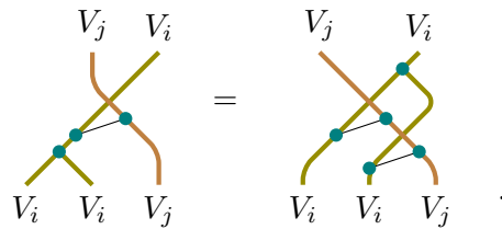
Figure 7.13: Naturality with respect to \mu_i .
