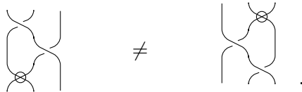
Figure 8.9: A forbidden mixed Yang-Baxter relation
