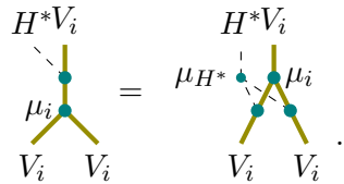
Figure 7.19: Compatibility for the left H^* -coaction
