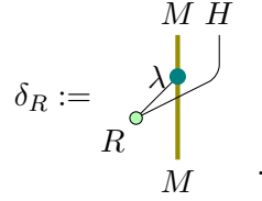
Figure 7.30: Action + R-matrix \mapsto coaction
