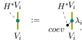
Figure 7.18: The duals come into play
