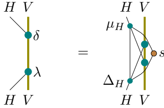
Figure 7.8: Left-left YD module
