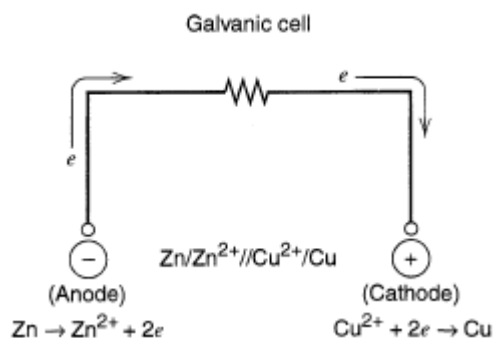
Fig. II. 1.2. Galvanic cell (Bard and Faulkner, 2001)
