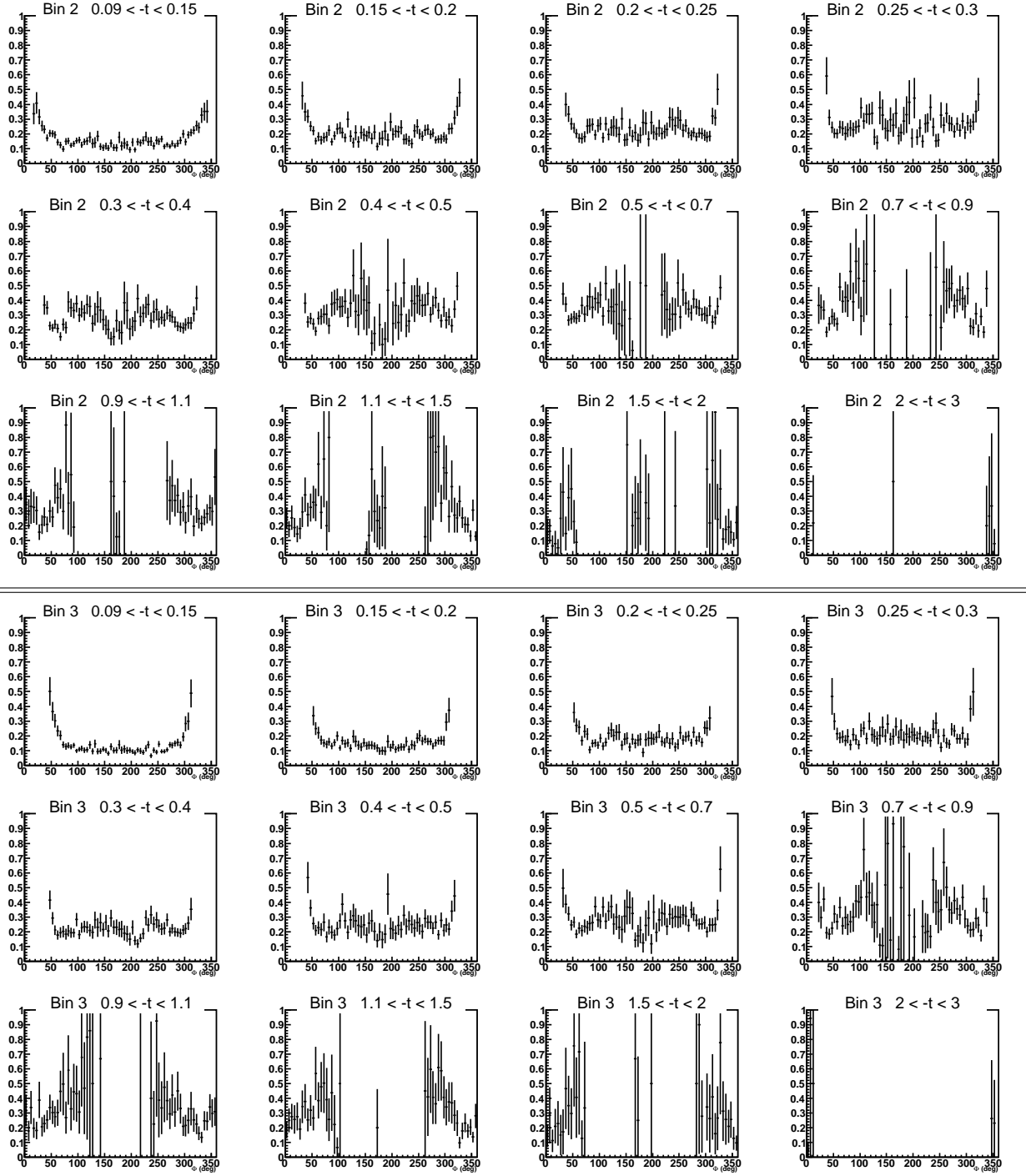
Figure F.2: \frac{N_{ep\pi^0(1\gamma)}}{N_{ep\gamma}} as a function of \Phi for the 12 t bins of the (Q^2, x_B) bins 2 and 3.
