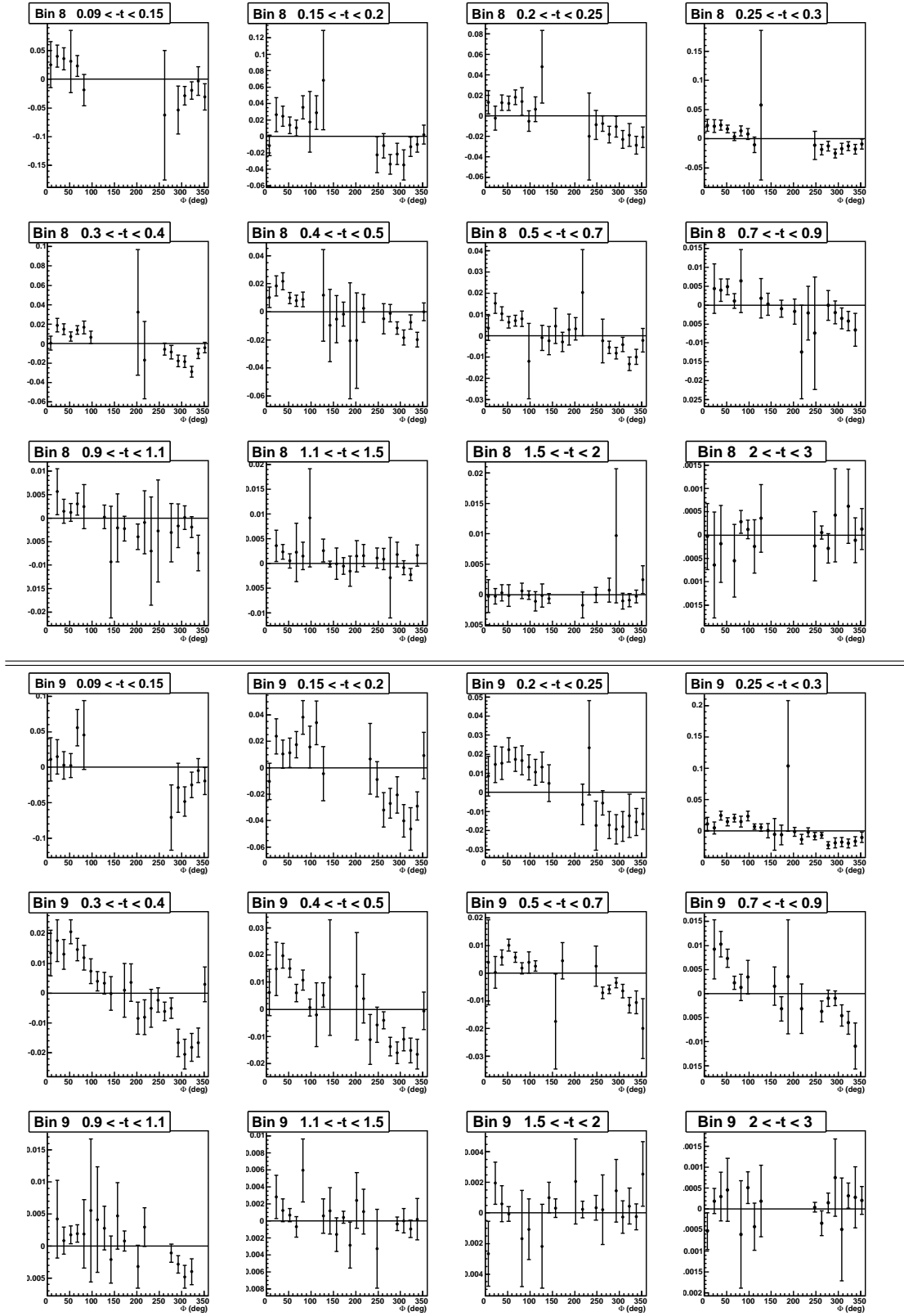
Figure I.5: Difference of polarized cross section as a function of \Phi for the 12 t -bins of the (Q^2, x_B) bins 8 and 9.
