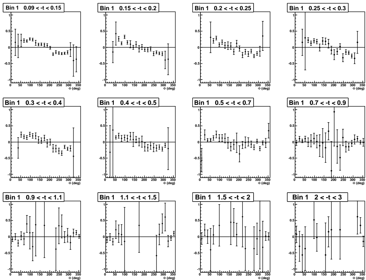
Figure K.1: Asymmetries as a function of \Phi for the 12 t -bins of the (Q^2, x_B) bin 1.
