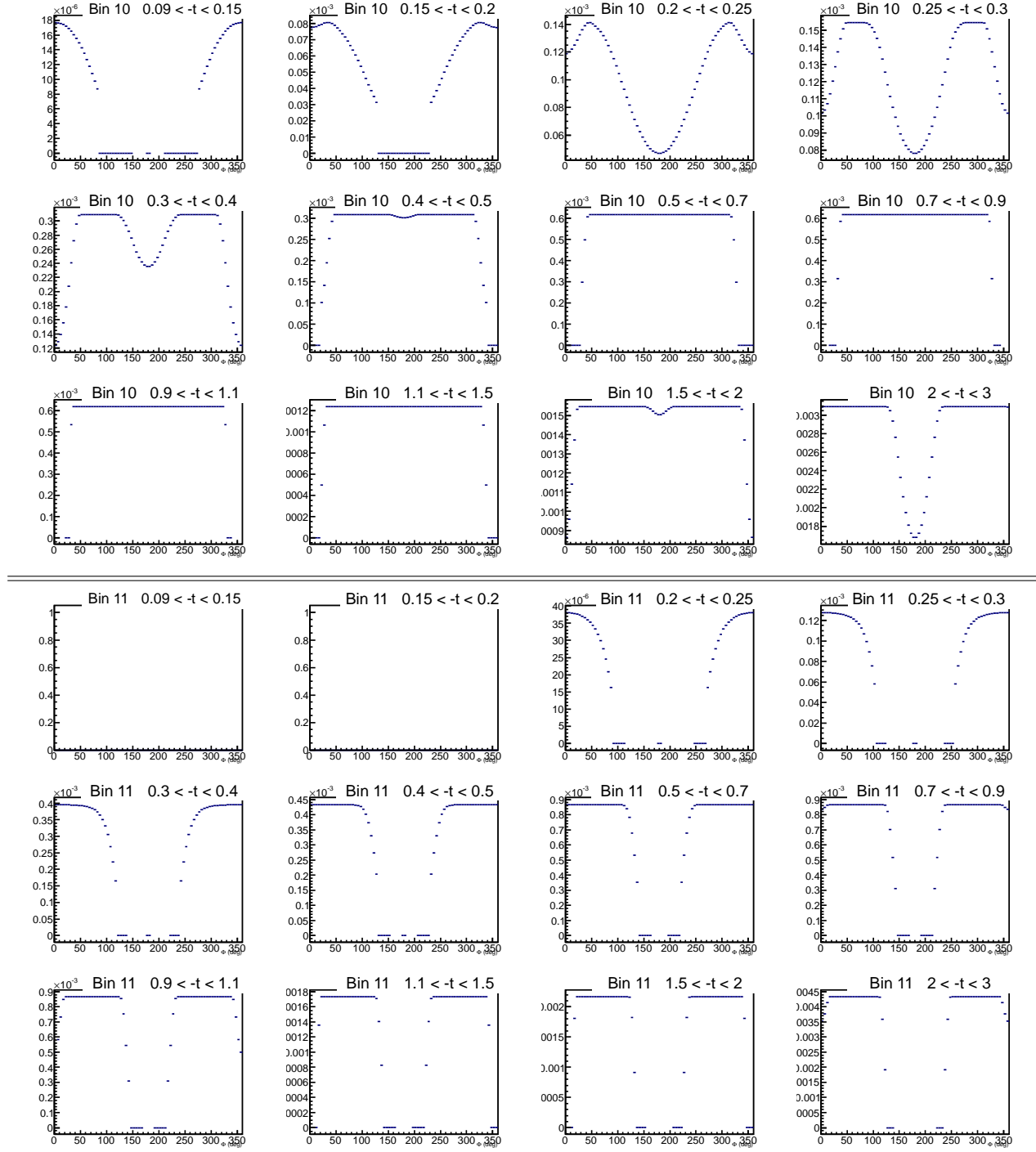
Figure E.6: Effective bin volume (GeV 4 rad) as a function of \Phi for the 12 t -bins of the (Q^2, x_B) bins 10 and 11.
