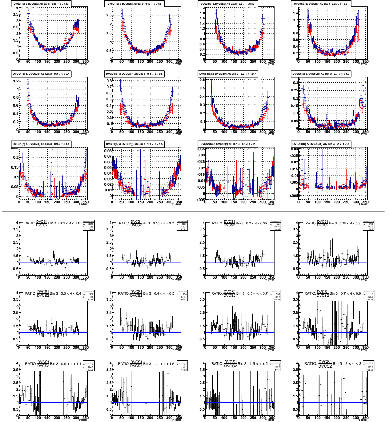
Figure H.3: Top: Comparison of the DVCS cross section for e1-DVCS1 (blue) e1-DVCS2 experiments. The cross section ( \text{nbarn}/\text{GeV}^4 ) are shown as a function of \Phi for the 12 t -bins of the (Q^2, x_B) bin 3. Bottom: ratio of the two experimental cross sections.
