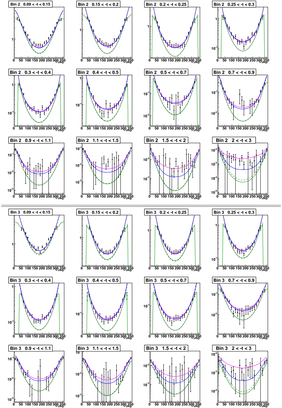
Figure L.2: DVCS cross section (nbarn/GeV 4 ) as a function of \Phi for the 12 t bins of the (Q^2, x_B) bins 2 and 3, compared to the BH cross-section and the VGG model predictions. The different curves are described in the text.
