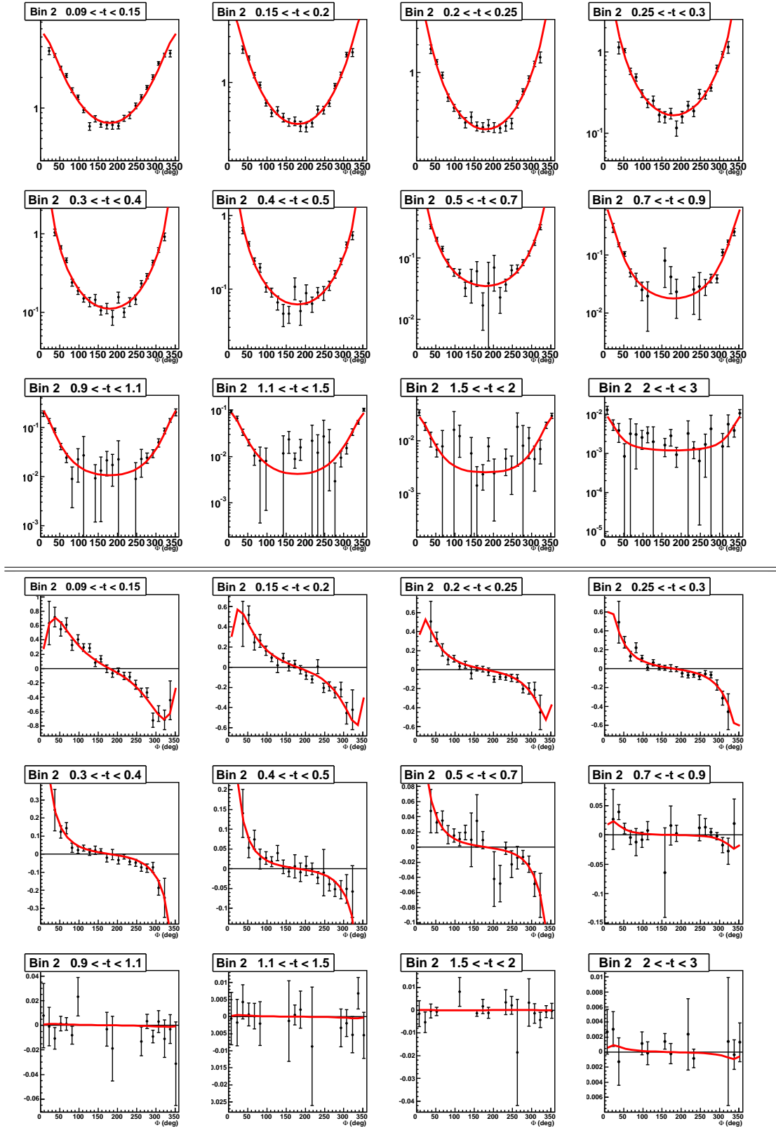
Figure O.2: Simultaneous fits of the unpolarized (top) and polarized (bottom) cross sections as a function of \Phi for the 12 t -bins of the (Q^2, x_B) bins 2.
