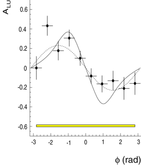
Figure 2.24: DVCS beam-spin asymmetry \mathcal{A}_{LU} as a function of the \phi angle (in radians) at the average kinematics \langle x_B \rangle = 0.11 , \langle Q^2 \rangle = 2.6 \text{GeV}^2 and \langle -t \rangle = 0.27 \text{GeV}^2 . The dashed line is a \sin \phi fit. The solid line is the theoretical GPD calculation of the VGG model with twist-3 effects [KPV01].
