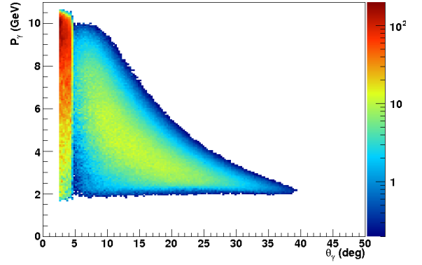
Figure 7.4: Photon momentum as a function of photon polar angle, for n -DVCS events. Forward-CLAS12 acceptance cuts and physics cuts are included.
