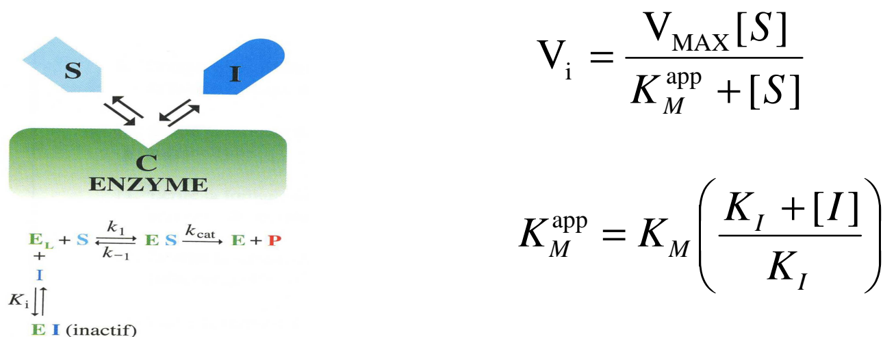
Figure 14 Inhibition compétitive
