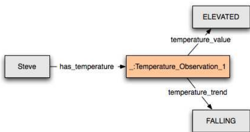
FIG. 1.2 – Représentation de la relation n-aire extraite de la phrase Steve has temperature, which is high, but falling (de Noy et Rector [2006]).
