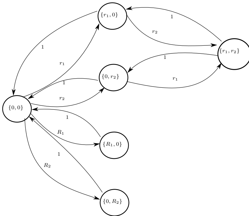
Figure 5.3: CMTTC modeling of the scheduling decisions. The scripts on the arrows indicate the transition rates.
