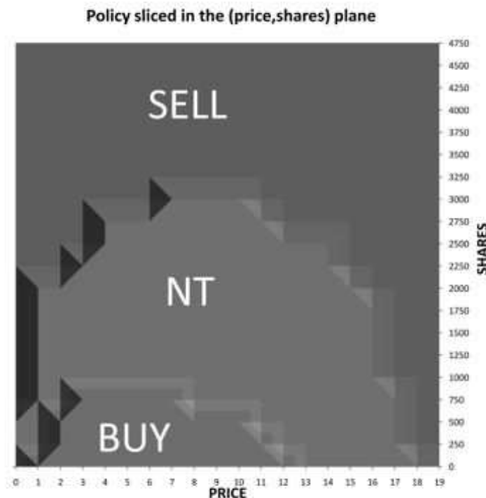
Figure 4.2: Test 1: Typical shape of the policy sliced in YP
