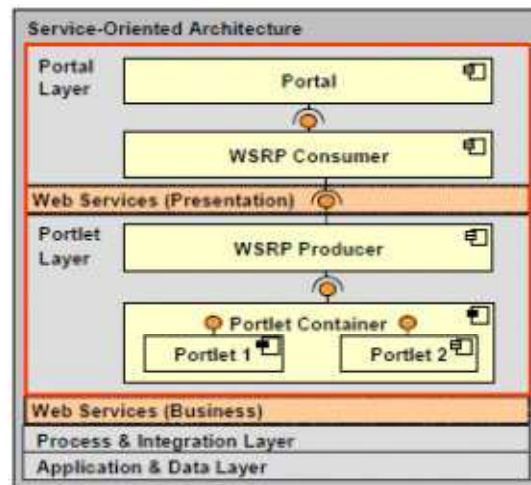
Figure 3.12. Architecture WSRP [Link et al.2006]
