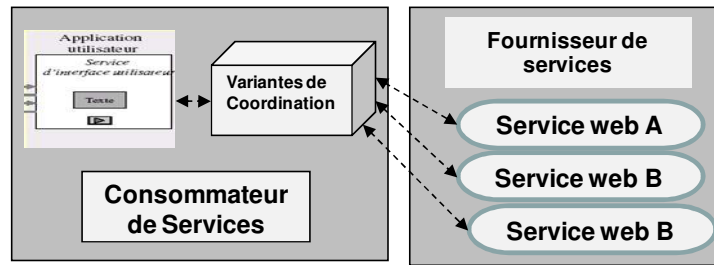
Figure 5.10. : Architecture 2-tier de composition interactive de service
