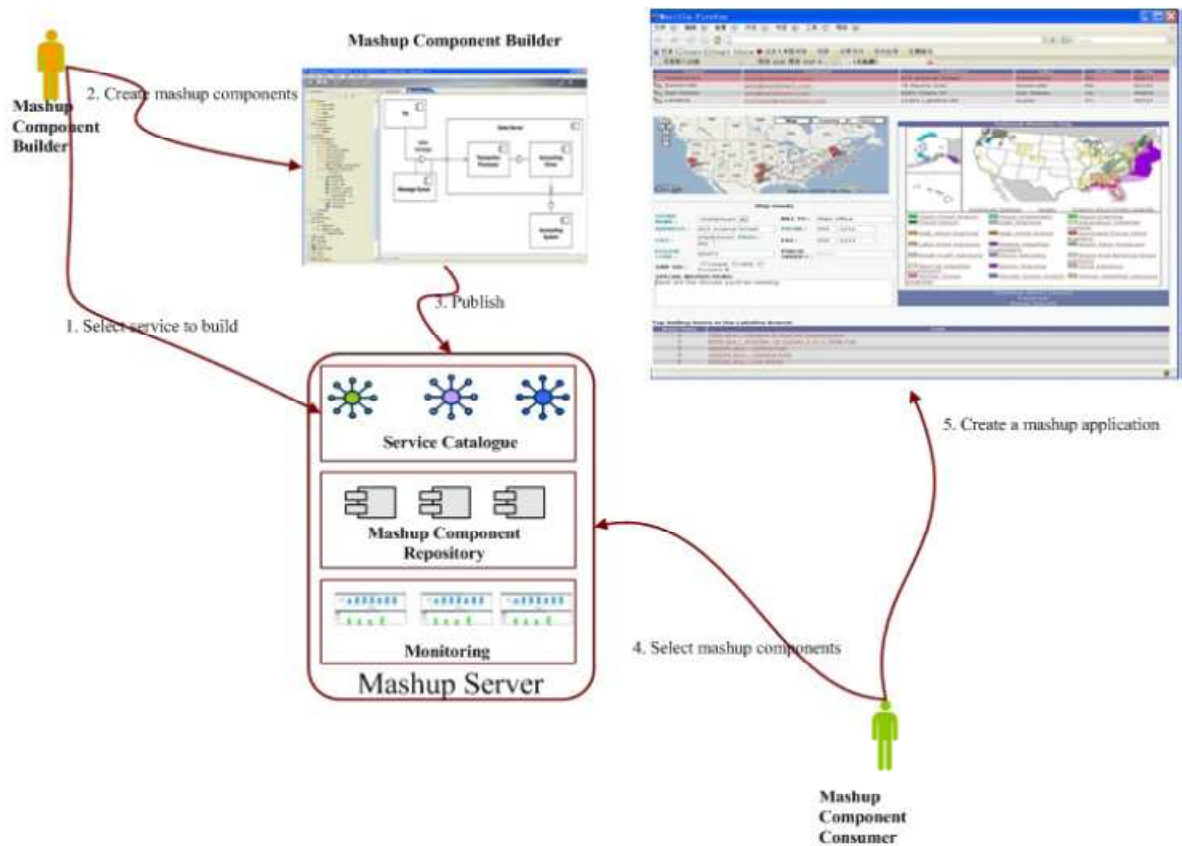
Figure 3.13. L'architecture Mashup
