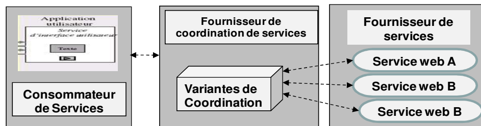
Figure 5.9. : Architecture 3-tier de composition interactive de service
