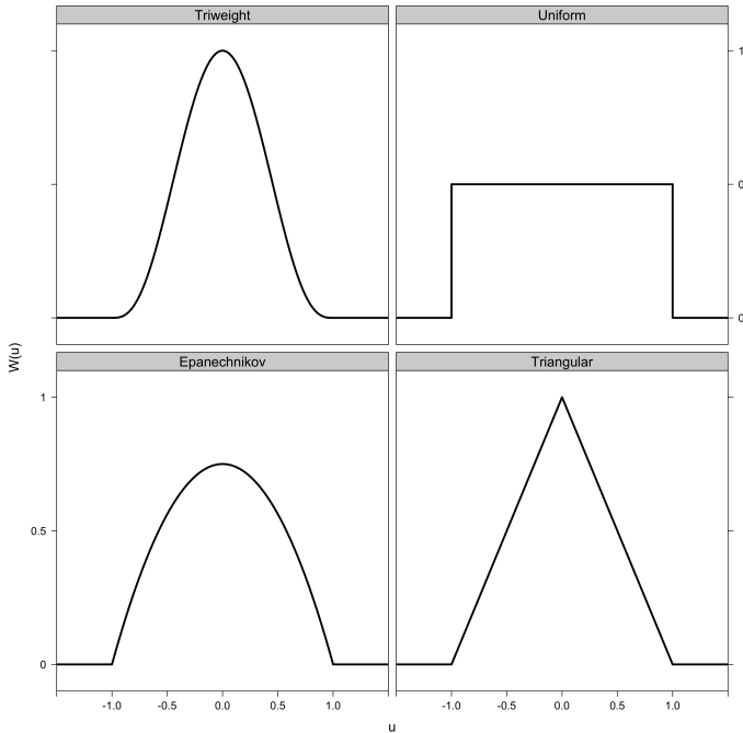
Figure 2.1: Weighting system shape of some weight functions.
