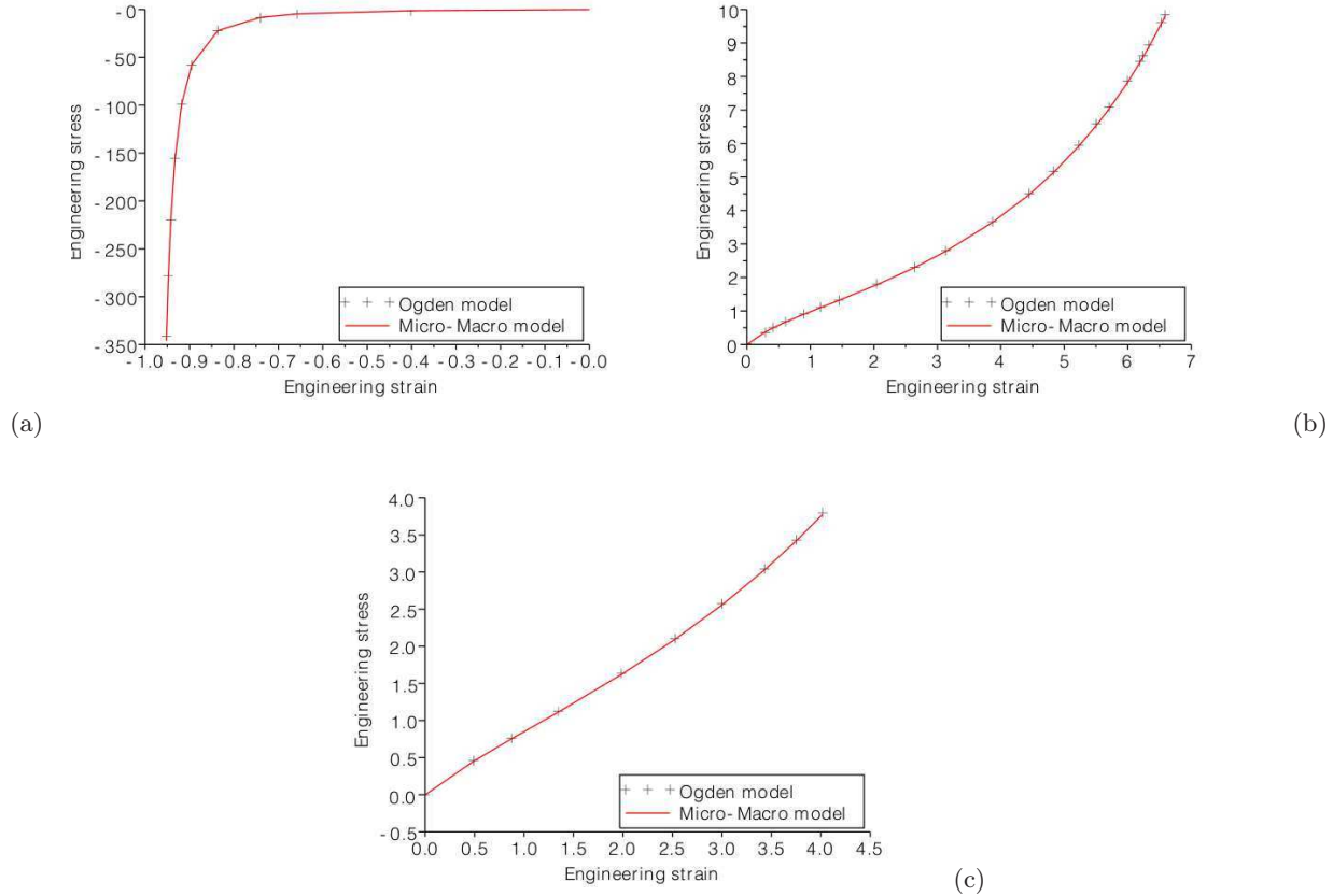
Fig. 4.16. Comparison between the discrete model for rubber and the reconstructed Ogden law. (a) uniaxial compression (b) uniaxial traction \xi = \text{diag}(\lambda, \frac{1}{\sqrt{\lambda}}, \frac{1}{\sqrt{\lambda}}) and (c) planar tension \xi = \text{diag}(\lambda, \frac{1}{\lambda}, 1) . Evolution of the engineering stress with respect to the engineering strain \lambda - 1 .
