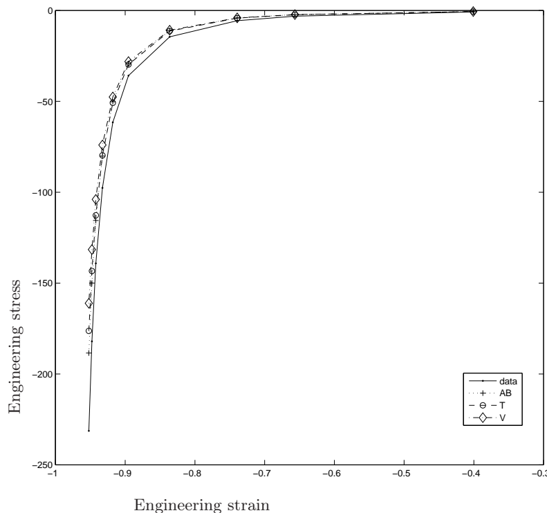
Fig. 4.10. Biaxial tension — Treloar’s experiments (AB: Arruda-Boyce, T: Treloar, V: variational — or homogenized)
