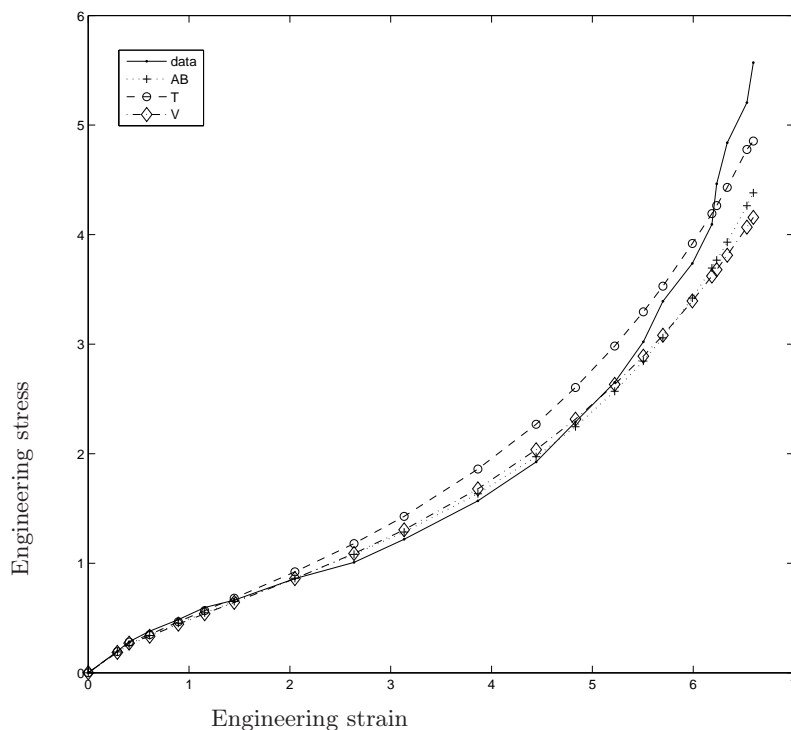
Fig. 4.9. Uniaxial traction — Treloar’s experiments (AB: Arruda-Boyce, T: Treloar, V: variational — or homogenized)
