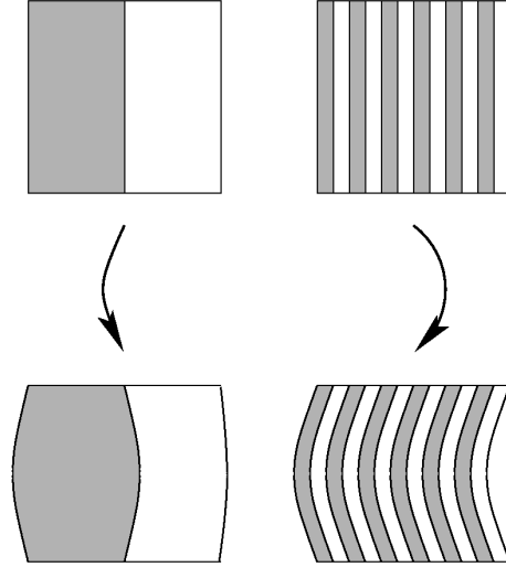
Fig. 3.1. Compression of one periodic cell and buckling of several periodic cells
