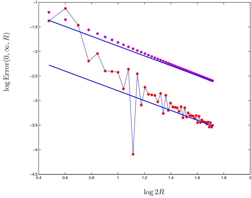
Fig. 2.6. Error in log-log for (2.43) in function of the number of cells per dimension 2R \in [3, 52] without zero-order term, with and without filtering: Slope -1 in both cases.
