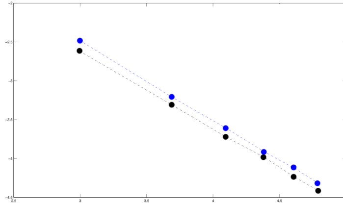
Fig. 1.1. Errors \langle |A_{\#}^N - A_{\text{hom}}|^2 \rangle^{1/2} (black) and \langle |A^{N,N} - A_{\text{hom}}|^2 \rangle^{1/2} (blue) in logarithmic scale
