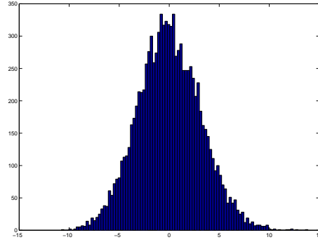
Fig. 1.5. Histogram of the rescaled fluctuations for t = 20
