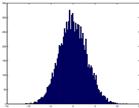
Fig. 1.4. Histogram of the rescaled fluctuations for t = 10
