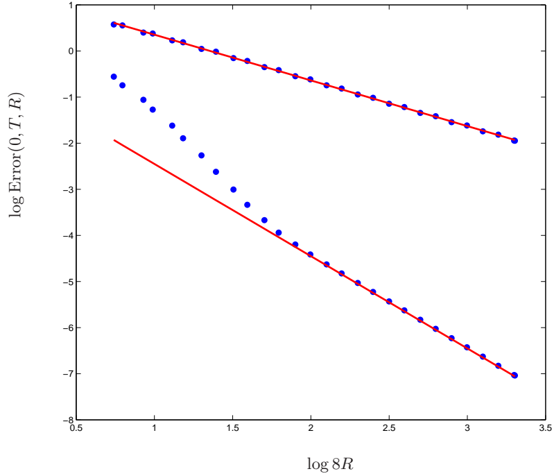
Fig. 2.3. Absolute error in log scale for T = 2R/25 , no filter (slope -1 ), infinite order filter (slope -2 ).
