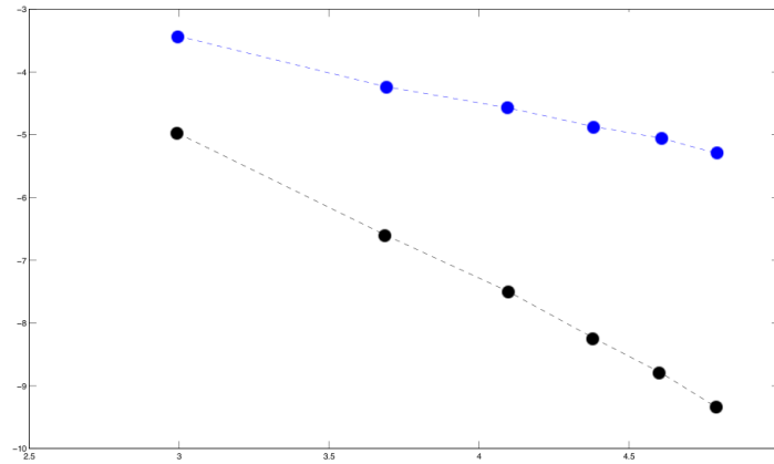
Fig. 1.2. Systematic errors |\langle A_{\#}^N \rangle - A_{\text{hom}}| (black) and |\langle A^{N,N} \rangle - A_{\text{hom}}| (blue) in logarithmic scale
