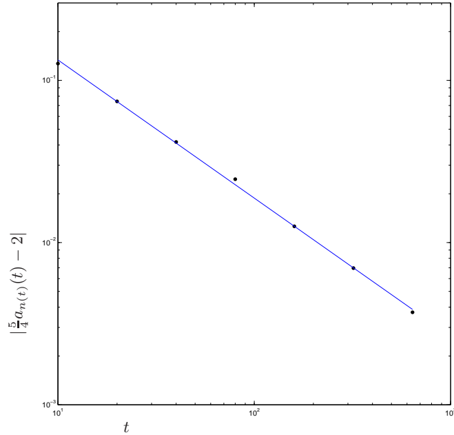
Fig. 1.3. Systematic error in function of the final time t for n(t) = K(t)t^2 realizations
