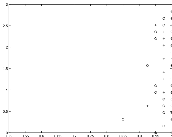
Fig. 2.10. Points chosen by the greedy algorithm for p = 41 and \bar{h}_1 = 1/40 (all the points chosen in [0, 1] \times [0, 2\pi] lie in [0.5, 1] \times [0, \pi] ).
