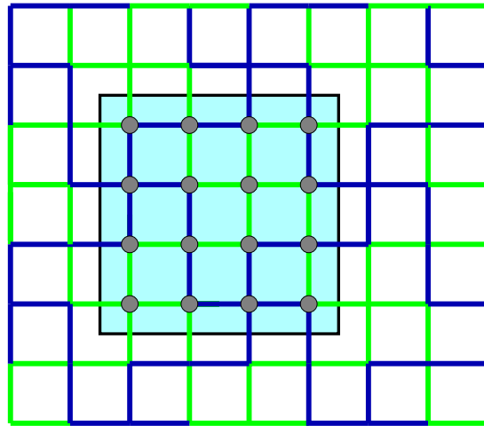
Fig. 2.1. Periodic cell in the discrete case
