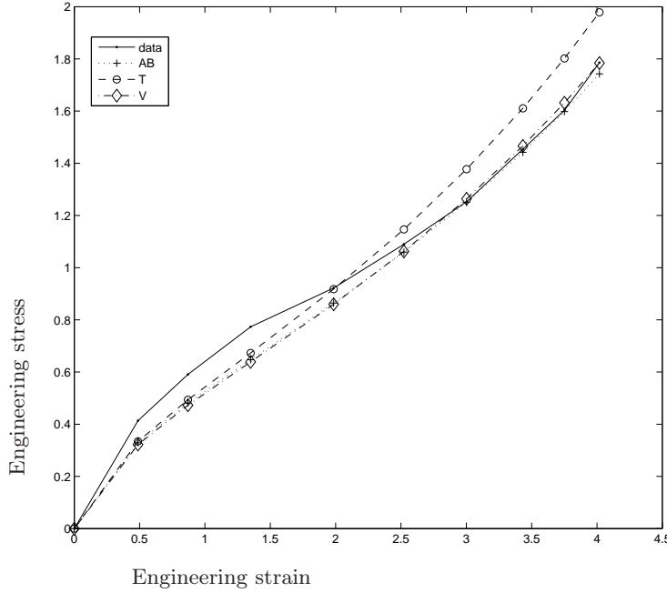
Fig. 4.11. Planar tension— Treloar’s experiments (AB: Arruda-Boyce, T: Treloar, V: variational — or homogenized)
