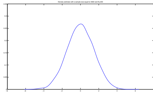
Fig. 1.11. Distribution of L^{d/2}(A_{\#}^L - \langle A_{\#}^L \rangle) around its expectation for L = 100
