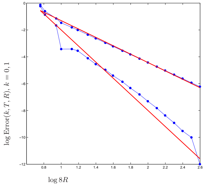
Fig. 2.5. Absolute error in log scale for T = (8R)^{3/2}/1000 , A_{0,T,L}^R (slope -3.1 ) and A_{1,T,L}^R (slope -6 ), filter of infinite order.
