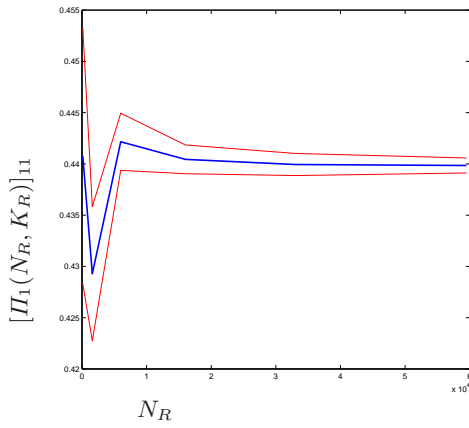
Fig. 4.3. Convergence of the diagonal part 1 of the Piola stress tensor for \Lambda_1
