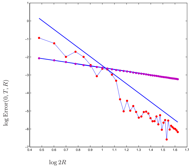
Fig. 2.9. Error in log-log for (2.44) in function of the number of cells per dimension 2R \in [3, 42] with a zero-order term T = R/100 , with and without filtering: Slopes -1 and -5 .
