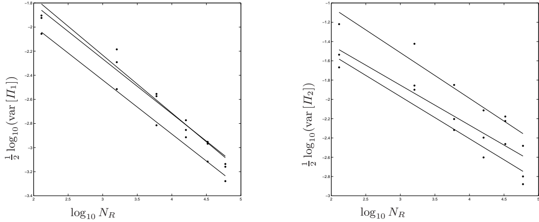
Fig. 4.1. Variance of the diagonal terms of the Piola stress tensor for \Lambda_1 Fig. 4.2. Variance of the diagonal terms of the Piola stress tensor for \Lambda_2
