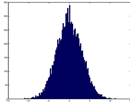
Fig. 1.5. Histogram of the rescaled fluctuations for t = 20
