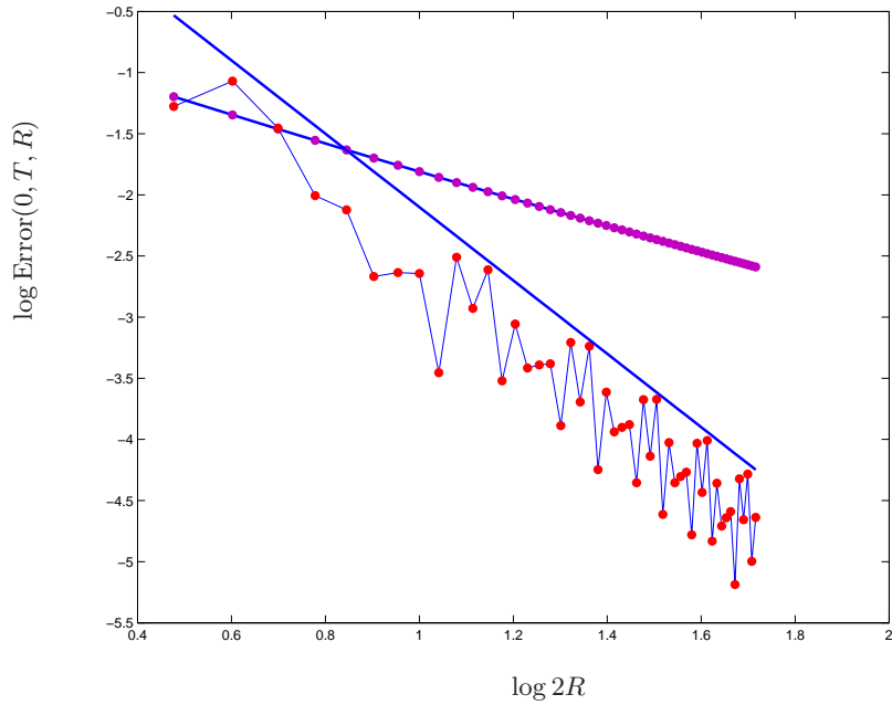
Fig. 2.7. Error in log-log for (2.43) in function of the number of cells per dimension 2R \in [3, 52] with a zero-order term T = R/5 , with and without filtering: Slopes -1 and -3 .
