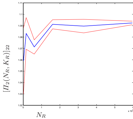
Fig. 4.7. Convergence of the diagonal part 2 of the Piola stress tensor for \Lambda_2
