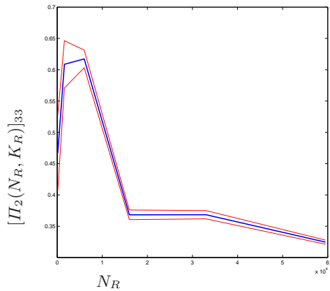
Fig. 4.8. Convergence of the diagonal part 3 of the Piola stress tensor for \Lambda_2
