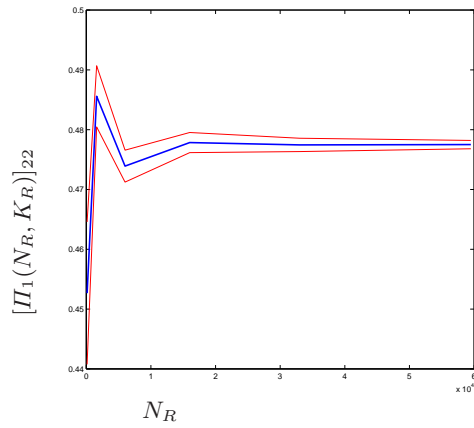
Fig. 4.4. Convergence of the diagonal part 2 of the Piola stress tensor for \Lambda_1
