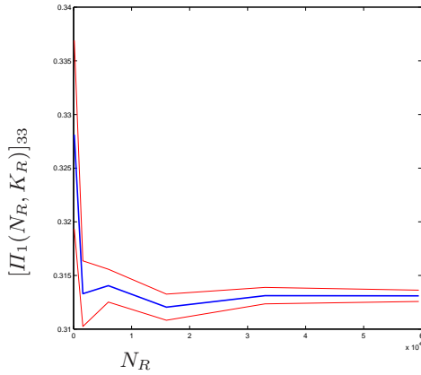
Fig. 4.5. Convergence of the diagonal part 3 of the Piola stress tensor for \Lambda_1
