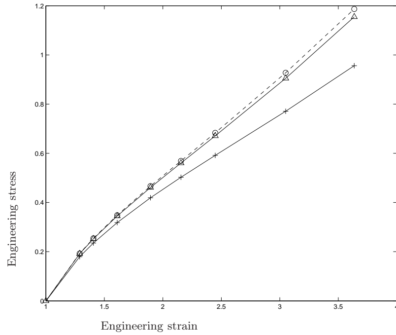
Fig. 4.17. Uniaxial traction — affine assumption (dashed line), variational model for K = 50 and connectivities 20 and 4 (from top to bottom)
