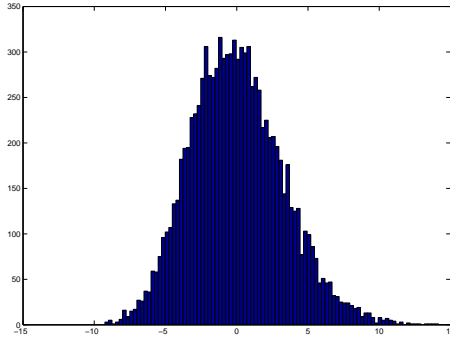
Fig. 1.4. Histogram of the rescaled fluctuations for t = 10
