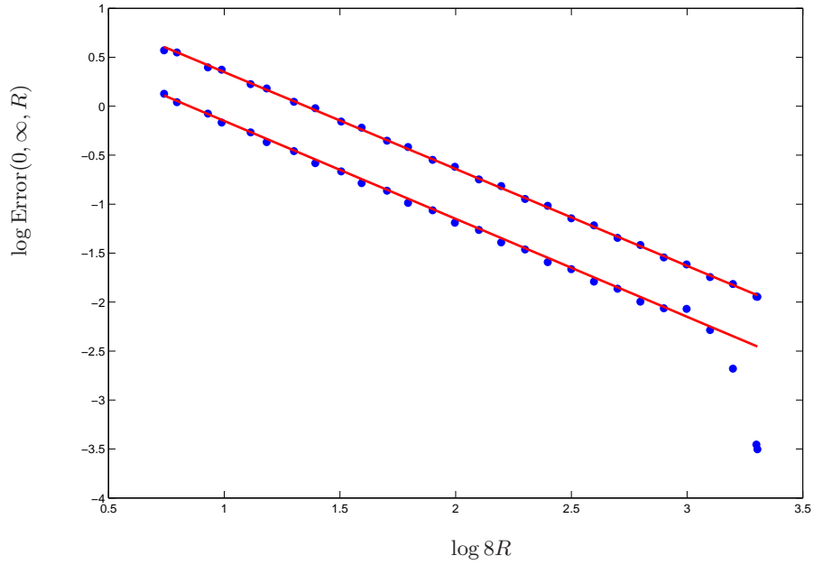
Fig. 2.2. Absolute error in log scale without zero order term, no filter (slope -1 ), infinite order filter (slope -1 , better prefactor).
