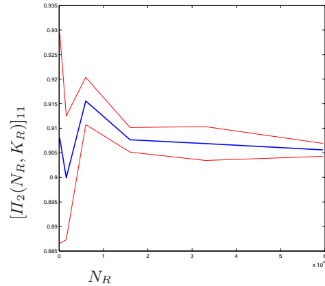
Fig. 4.6. Convergence of the diagonal part 1 of the Piola stress tensor for \Lambda_2
