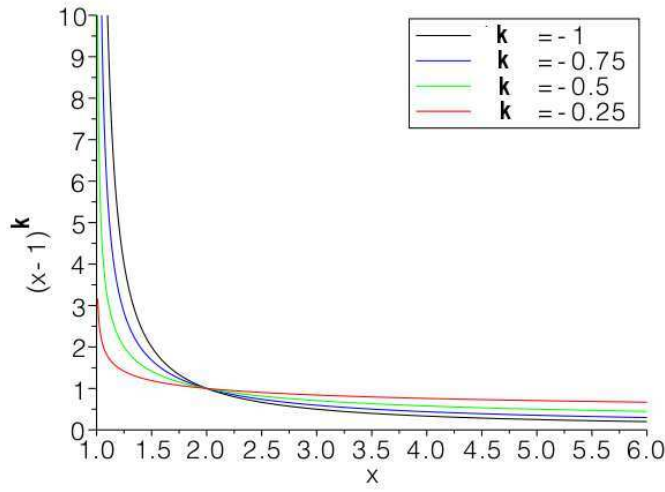
Fig. 4.15. Jacobi weight function x \mapsto (x - 1)^\kappa (for \kappa \in \{-1, -0.75, -0.5, -0.25\} )
