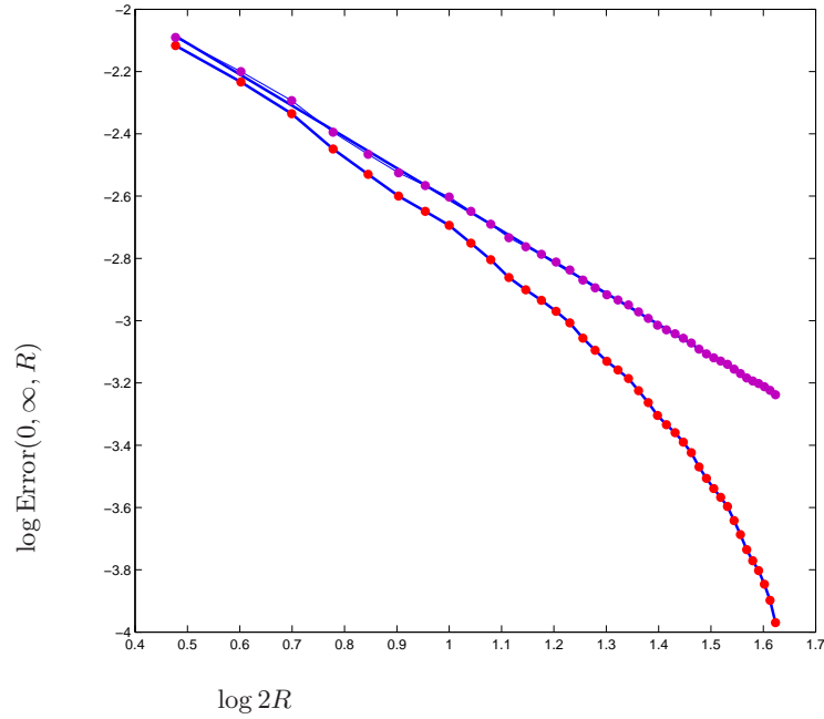
Fig. 2.8. Error in log-log for (2.44) in function of the number of cells per dimension 2R \in [3, 42] without zero-order term and without filtering, for the two different coefficients of reference: Slope -1 and artificial super-linear convergence.
