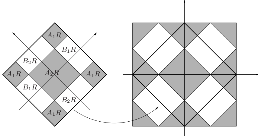
Fig. 3.3. The values of CR + \nabla\phi in R^{-1}(-1/\sqrt{2}, 1/\sqrt{2})^2 . On the left the axis are oriented in the directions R^{-1}\mathbf{e}_1 and R^{-1}\mathbf{e}_2 .
