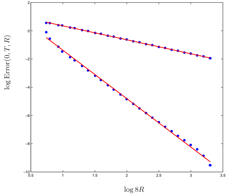
Fig. 2.4. Absolute error in log scale for T = (8R)^{7/4}/5000 , no filter (slope -1 ), infinite order filter (slope -3.4 ).
