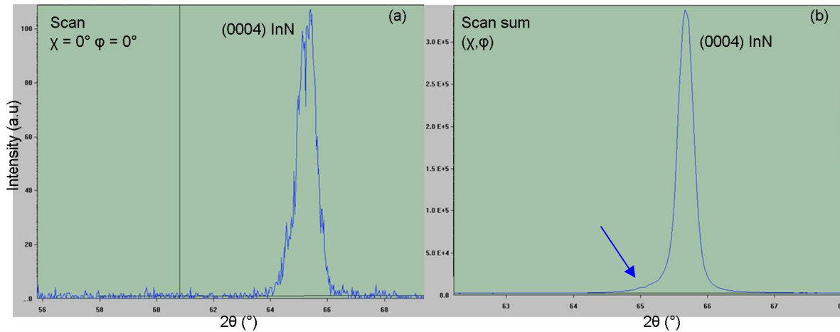
Fig 3.24 For (0004) InN reflection: (a) ( \chi, \phi ) scan with \chi = \phi = 0^\circ and (b) summed scan of all \chi and \phi angles showing the asymmetry at the left side of the peak (see arrow).
