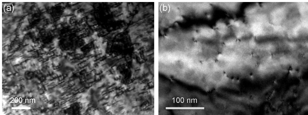
Fig 3.33 Plan view images on R512 sample: (a) bright field \mathbf{g} = \langle \bar{1}\bar{2}\bar{1}\bar{3} \rangle zone axis image - all type dislocations are visible, (b) \mathbf{g} = \langle \bar{1}\bar{1}\bar{2}0 \rangle zone axis - edge and mixed dislocations are visible.
