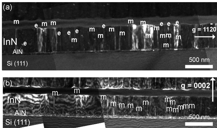
Fig 3.30 Cross-section micrograph of sample R117 (InN/AlN/Si (111)) taken under (a) \mathbf{g} = 11\bar{2}0 and (b) \mathbf{g} = 0002 , both in dark field mode. Mainly, mixed (m) and edge (e) dislocations are observed in these images, and no screw dislocations can be noticed.
