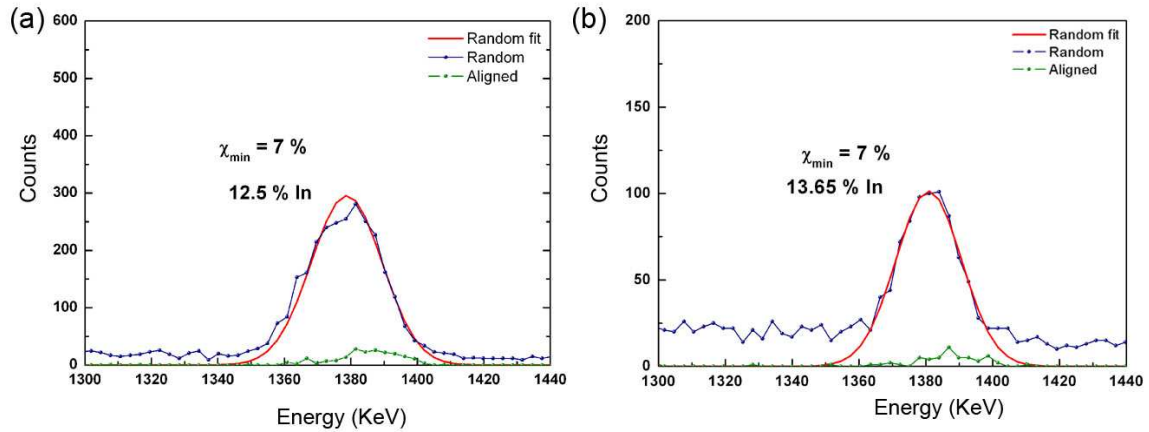
Fig 4.14 RBS/C random and <0001> aligned spectra for the In signal: (a) Aix3232, and (b) Aix3234.
