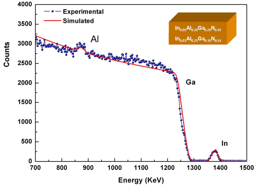
Fig 4.33 RBS spectra and simulated including Ga in the caplayer. Schematic structure of the two InAlGaN layers fitted in SIMNRA is also given.
