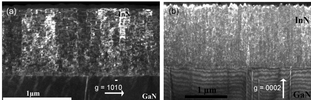
Fig 3.2 Cross sectional TEM images: (a) sample 1269, \mathbf{g} = 10\bar{1}0 (high density of stacking faults), (b) sample 1273, \mathbf{g} = 0002 .
