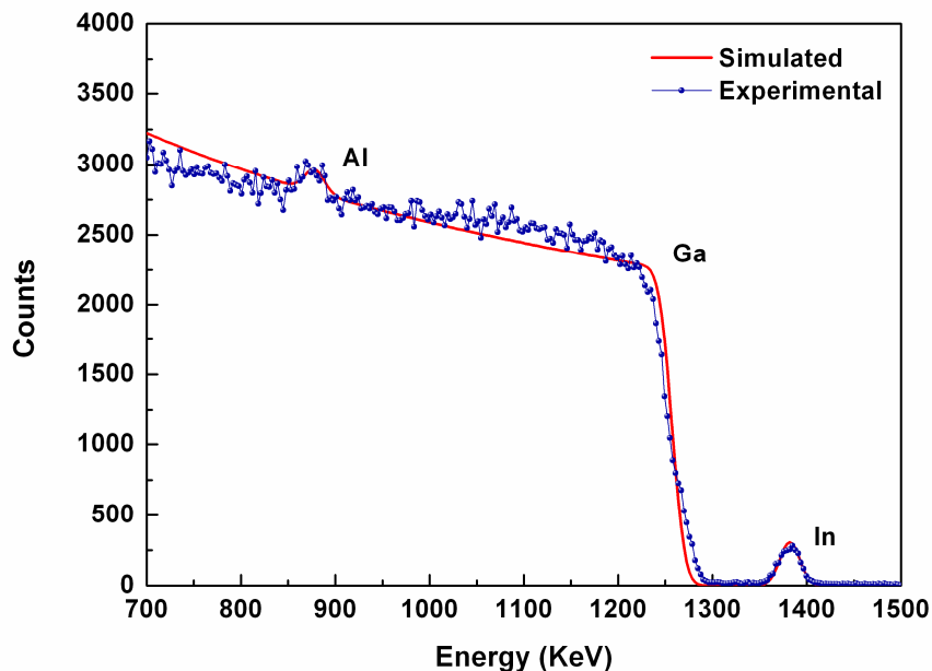
Fig 4.31 RBS experimental and simulated spectra using \text{In}_{0.06}\text{Al}_{0.42}\text{N}_{0.52}/\text{GaN} heterostructure for Aix3232.
