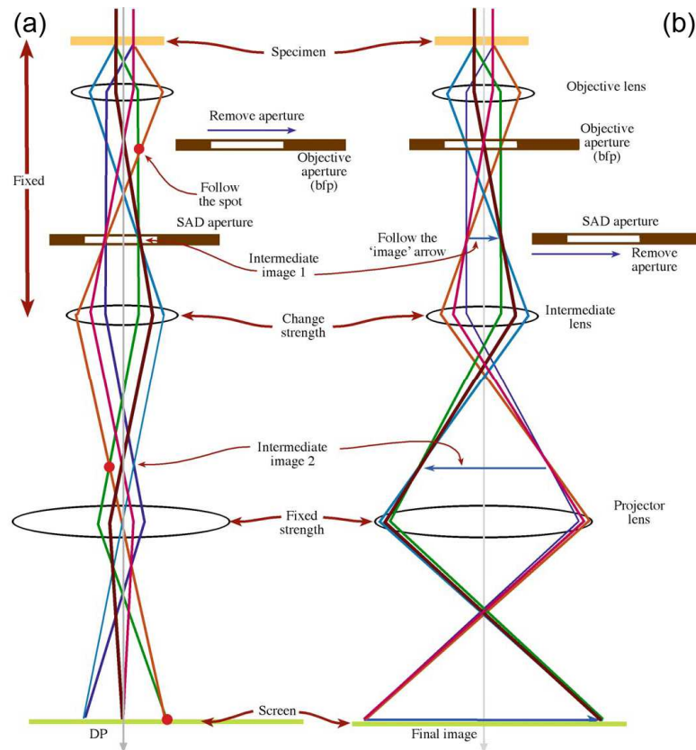
Fig 2.5 The two basic operations of TEM imaging system (a) diffraction pattern (b) image code. 12
