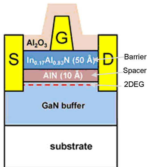
Fig 1.2 Schematic cross section of In 0.17 Al 0.83 N/AlN/GaN HEMT. 24
