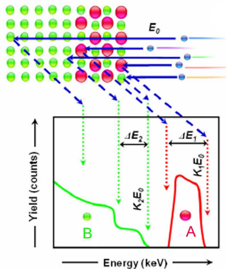
Fig 2.14 Representation of an RBS spectrum for the simple case of two layers. 19
