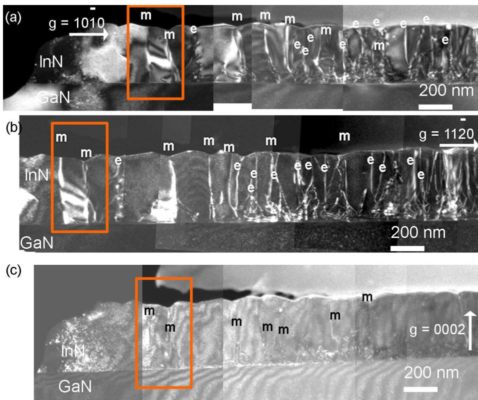
Fig 3.29 Cross-section TEM images of InN/GaN (R593) taken under (a) g = 10\bar{1}0 dark field image (b) g = 11\bar{2}0 dark field image and (c) g -3 g weak beam with g = 0002 image diffraction conditions. Only edge (e) and mixed (m) TD density were identified on these micrographs.
