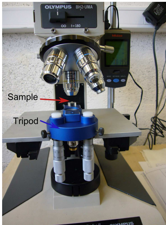
Fig 2.10 Tripod used for the sample preparation.
