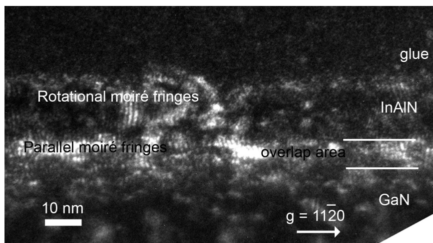
Fig 4.3 Moiré fringes in sample Aix3235 ( t_{\text{AlN}} = 6.9 \text{ nm} ).
