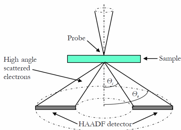
Fig 2.8 Schematic of the STEM-HAADF system configuration. The probe is rastered across the sample and high angle scattered electrons are collected by an annular detector with an inner collection angle \theta_i and an outer collection angle \theta_o .
