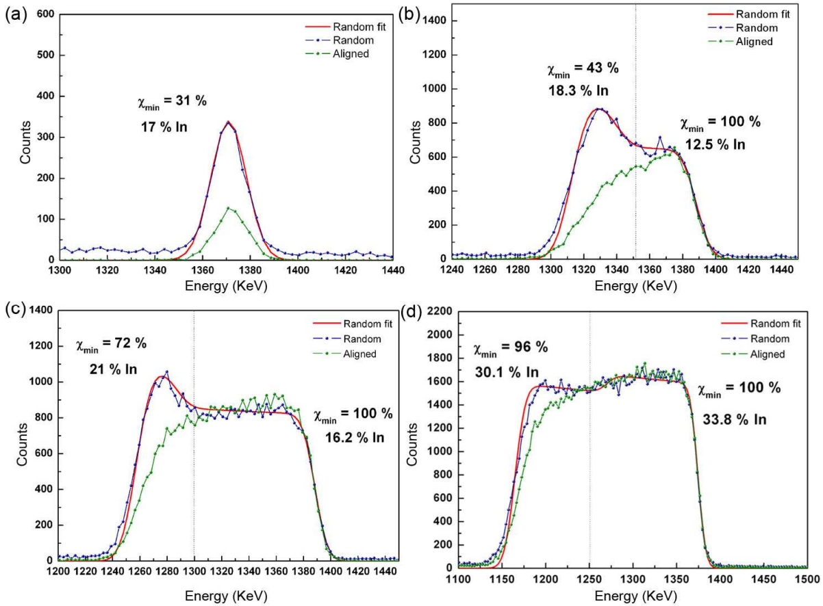
Fig 4.15 RBS random and \langle 0001 \rangle aligned spectra of samples: (a) AEC1769, t_{\text{InAlN}} = 7.9 \text{ nm} (b) AEC1657, t_{\text{InAlN}} = 100 \text{ nm} (c) AEC1655, t_{\text{InAlN}} = 150 \text{ nm} , and (d) AEC1323, t_{\text{InAlN}} = 260 \text{ nm} . Vertical dashed line separates the two layers used in the fit with different composition.
