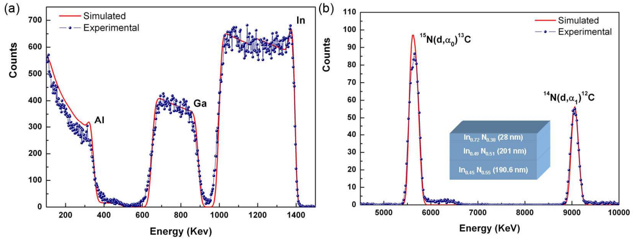
Fig 3.16 Ion beam analysis in R135 sample: (a) experimental (blue circles) and simulated (red solid line) RBS spectra of InN film (b) NRA spectrum, a schematic structure of the three InN layers fitted in SIMNRA is inserted.
