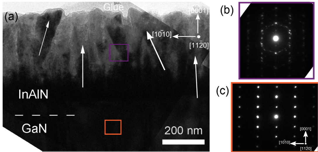
Fig 4.9 Sample AEC1323 (a) Cross section at the [1\bar{1}20] zone axis; (b) and (c) [1\bar{1}20] diffraction pattern taken from InAlN and GaN layer.
