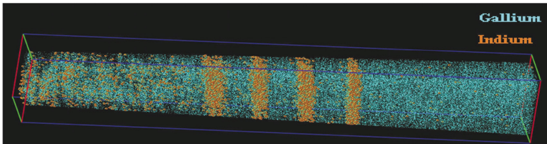
Figure 4. 4. Three-dimensional Atom Probe Field Ion Microscope (3DAP) image of \text{InGaN/GaN} multi quantum wells. Each dot represents a single atom: light blue is Gallium and orange is Indium 32 .
