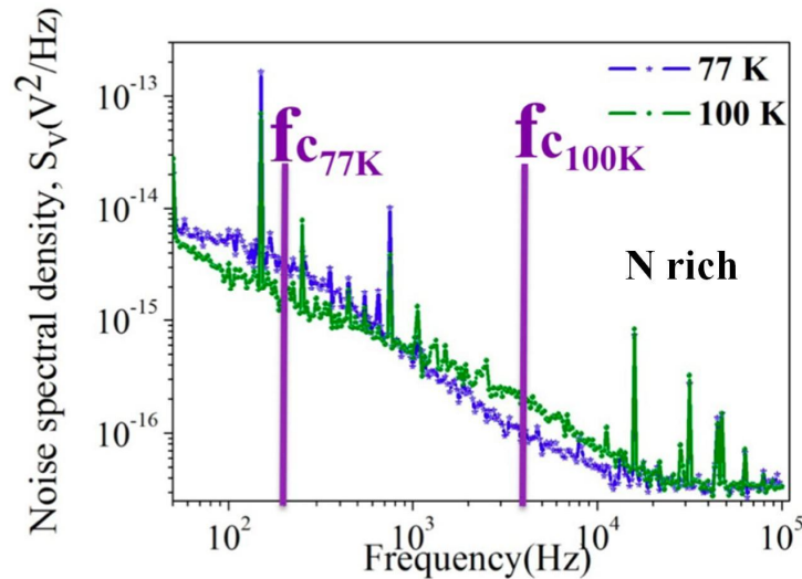
Figure 3. 20. Characteristic lorentzian frequency variation with temperature (sample B3): f_c _{77K} , f_c _{100K} are the lorentzian frequencies for sample B3.
