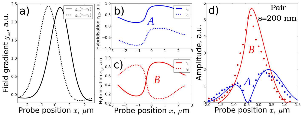
Figure 6.9: a) Stray field g_{zz} at the probe location from two uncoupled discs separated by 200 nm. b) and c) Coupled spin wave amplitude in each disc of the pair s = 200 nm versus probe position for the binding B and anti-binding A coupled modes. d) Amplitude of the coupled modes measured by f-MRFM (dots) and calculated (solid lines) as a function of the tip position for the pair separated by s = 200 nm. A corresponds to the optical mode while B is the acoustic mode.
