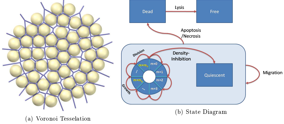
Figure B.1: A cell is defined by its position, its internal state and a set of transition rules.
