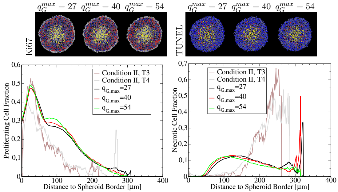
Figure 4.18: Sensitivity analysis for glucose consumption parameter q_{G,max} . The collages for nutrimental condition III (a) and II (b) show the "stained" slices of in-silico spheroids when reached a radius of 300\mu m (top) and the radial profiles of the proliferating (left) and necrotic (right) cell fractions. The radial profiles emerging in-silico are compared to data. The simulations were done for different values of glucose consumption parameter q_{G,max} . The color code of the spheroid slices are: proliferating (red, Ki67), quiescent (blue, Ki67), necrotic (red, TUNEL), viable (blue, TUNEL) and the lysated cells (yellow)
