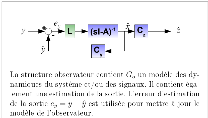
Figure 2.3 – Structure Observateur
