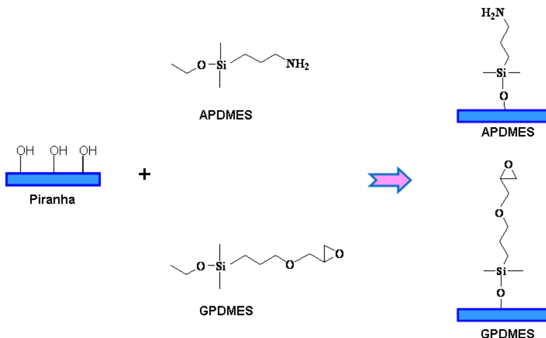
Figure 2-4 Schematic illustration of silanization with APDMES and GPDMES
