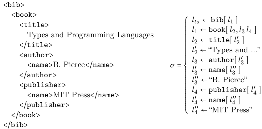
Figure 4.1: Document t_2 and store (\sigma, l_{t_2})
