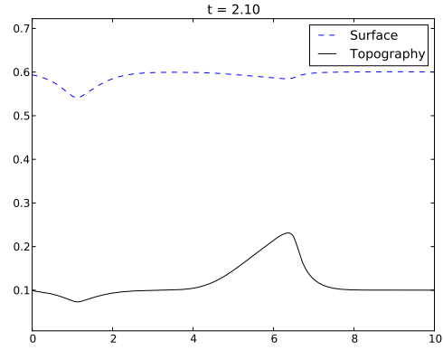
(b) Splitting scheme CFL = 0.5
