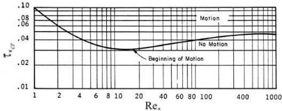
Figure 1.4: Shields's diagram [159].
