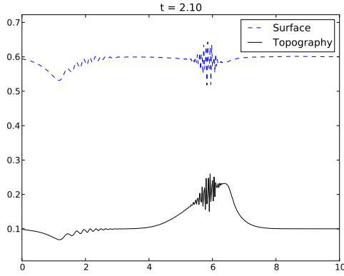
(a) Splitting scheme CFL = 0.95
