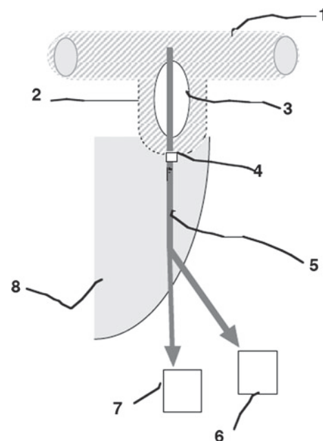
Fig. 3 Intrapulmonary pulsatile system. 1 pulmonary artery branch, 2 pulmonary artery trunk, 3 inflated balloon in place, 4 infundibular snugger, 5 catheter shaft, 6 cardiopulmonary monitor, 7 pulsatile driving system (small animal ventilator), 8 right-ventricular cavity
