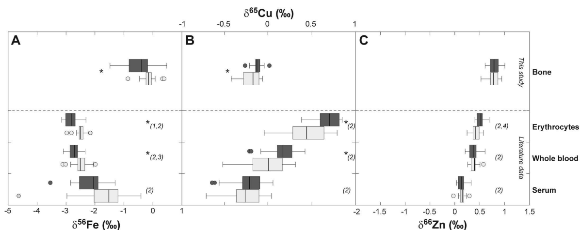
FIGURE 10.2.1: Fe, Cu and Zn isotope variations of the organs discussed in the text. The delta annotations are given by \delta^x Fe = \left[ \frac{(^x Fe / ^{54} Fe)_{sample}}{(^x Fe / ^{54} Fe)_{standard}} - 1 \right] * 1000 with x = 56 or 57 ). The “IRMM14” solution stands for the Fe isotope standard. \delta^{65} Cu = \left[ \frac{(^{65} Cu / ^{63} Cu)_{sample}}{(^{65} Cu / ^{63} Cu)_{standard}} - 1 \right] * 1000 . The “NIST-SRM 976” solution was used as Cu isotope standard. \delta^x Zn = \left[ \frac{(^x Zn / ^{64} Zn)_{sample}}{(^x Zn / ^{64} Zn)_{standard}} - 1 \right] * 1000 with x = 66, 67, 68, or 70 ). The “JMC 3-0749” solution is the well-distributed Lyon Zn isotope standard. The box represents the 25th–75th percentiles (with the median as a bold vertical line) and the whiskers show the 10th–90th percentiles. Numbers in brackets correspond to references. Bone data are from this study. Statistically significant differences between women and men ( p < 0.02 ) are indicated by an asterisk. Literature data : 1. Walczyk and von Blanckenburg, 2002. ; 2. Albarède et al, 2011 ; 3. Ohno et al, 2004 ; 4. Ohno et al, 2005.
