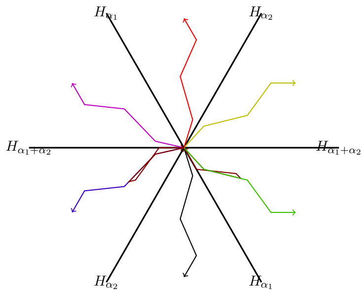
Figure 2.8: A_2 -type path crystal for highest weight \lambda = \rho = \alpha_1 + \alpha_2
