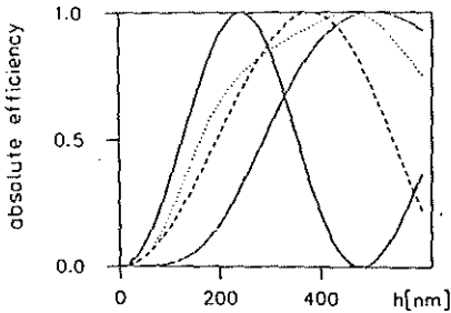
Fig.9.1. Groove depth dependence of -1st order efficiency of dielectric grating with light incident from the substrate side ( n=1.5 ). Solid line - TE polarization (polarization) ( \lambda=0.550 \mu\text{m} ), dotted curve - TM polarization ( \lambda=0.550 \mu\text{m} ); dashed line - TE polarization ( \lambda=0.650 \mu\text{m} ), border line - TM polarization ( \lambda=0.650 \mu\text{m} ). d=0.26 \mu\text{m} , Littrow mount.
