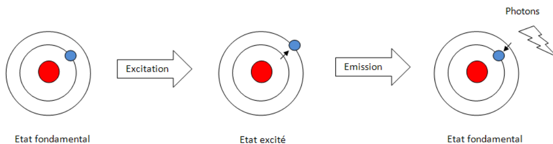
Figure 8: Emission atomique
