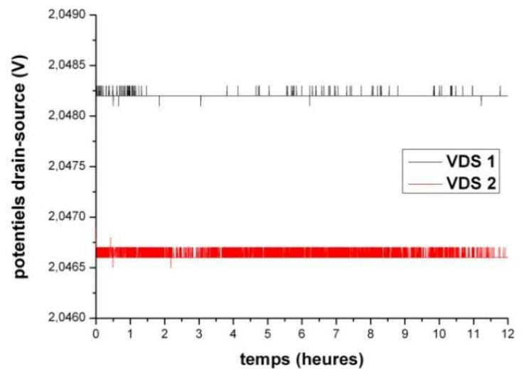
Figure 10: potentiels drain-source
