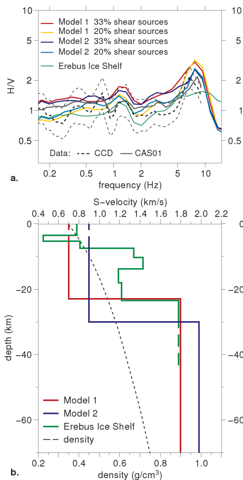
Figure 4.3: (a) Fit of the H/V spectral ratios at the Dome C stations CCD (dashed, with standard deviation) and at CAS01 (grey line), with two different models and two different compositions of the noise. Also shown is the result obtained for an Erebus ice shelf model. (b) S-wave velocity models used in (a) (scale at the top, model 1 preferred), and density profile at Concordia (L. Arnaud, personal communication 2010, scale at the bottom). L ev eque et al. (2010, Fig. 6)
