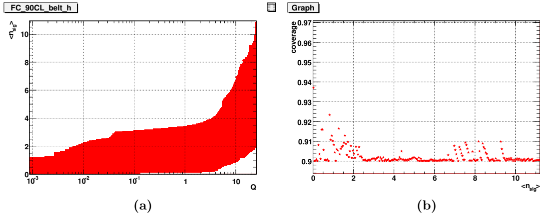
Figure 6.13: Feldman-Cousins 90%CL belt (a), note the Q in log scale, and coverage of the acceptance intervals (b). The coverage is stable up to 5\sigma levels.
