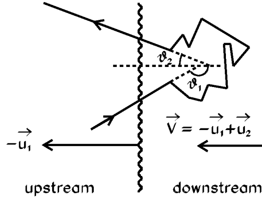
Figure 1.5: Plane shock for the first order Fermi acceleration. The shock front propagates to the left towards the unshocked upstream gas.
