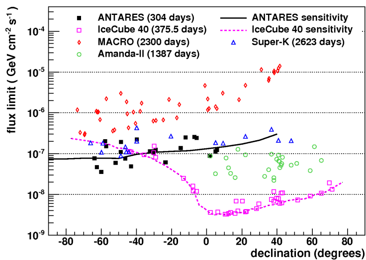
Figure 2.17: Top: sky map of the candidate neutrino events selected in the 2007-2008 data (blue squares), used for the search of point-like neutrino sources. The red circles represent the candidate sources. The red square indicates the most significant cluster of events obtained from the full sky search. Bottom: limits set on the normalization \phi of an E_\nu^{-2} spectrum of high-energy neutrinos from selected candidates. The points show the 90% CL limit at the declination of the candidate source. From (Adrián-Martínez et al., 2011a).
