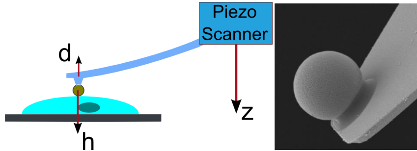
Fig. 4-4: AFM spherical probe for rheological study
