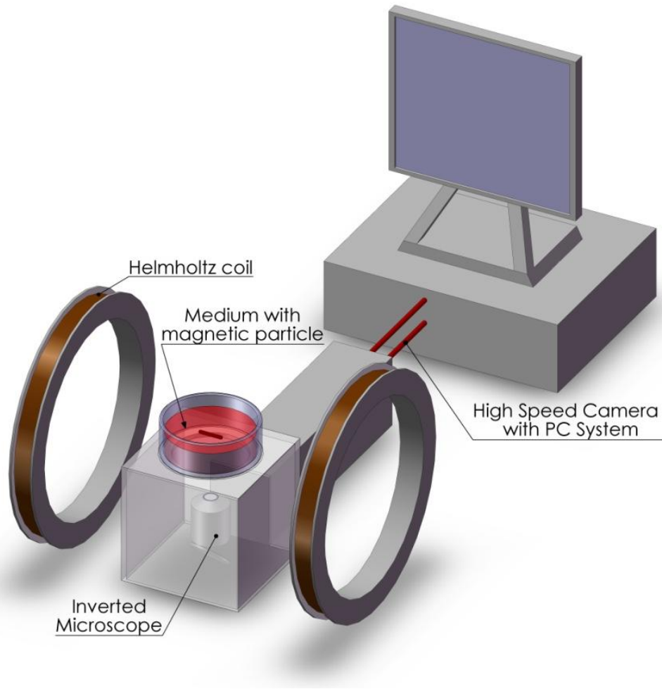
Fig. 3-1 : Experimental setup
