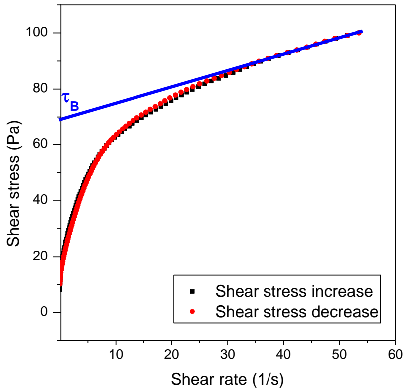
Fig. 3-13: Shear stress/shear rate of carbopol, measured by rotational rheometry; the blue line is a Bingham fit of the decreasing stress with \tau_B=70Pa and \eta=16.7 Pa
