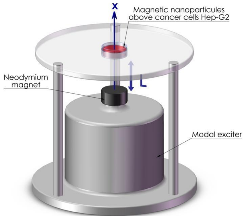
Fig. 6-1: Experimental setup
