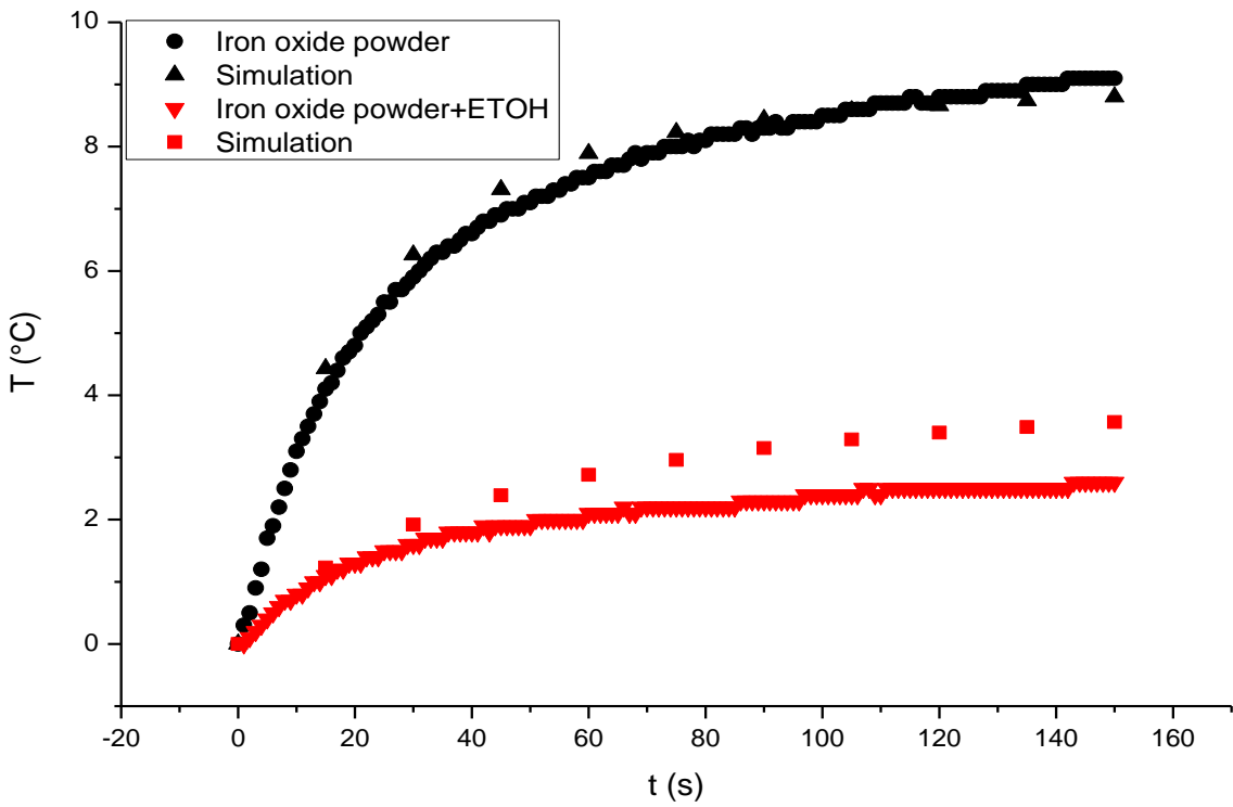
Fig. 7-8: Temperature rise versus time, comparison of experimental and simulation results for iron oxide powder with and without ethanol, the conditions of experiment: f=5 kHz, H=12 kA/m
