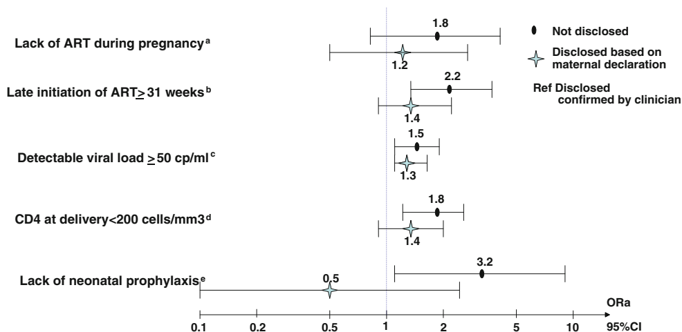
Fig. 1 Adjusted odds ratios (ORa) of non optimal PMTCT practices according to status for HIV disclosure to the partner, ANRS-EPF-CO1, 2005–2009. Adjusted on: a time of HIV diagnosis, b gestational age at booking and maternal occupational status, c late treatment and maternal occupational status, d maternal occupational status, e gestational age at delivery and maternal occupational status
