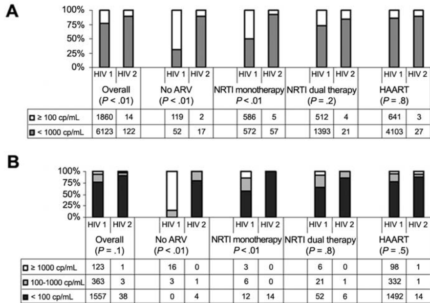
Figure 1. A, Mothers with available measurements of plasma human immunodeficiency virus (HIV) RNA for the overall period (1996–2007). B, Mothers with available measurements of plasma HIV RNA for the 2005–2007 period. ARV, antiretroviral therapy; cp, copies; HAART, highly active antiretroviral therapy; NRTI, nucleoside reverse-transcriptase inhibitor.
