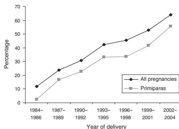
Fig. 1. Evolution of the proportion of pregnancies in sub-Saharan African immigrants in the ANRS EPF, 1984–2004.
