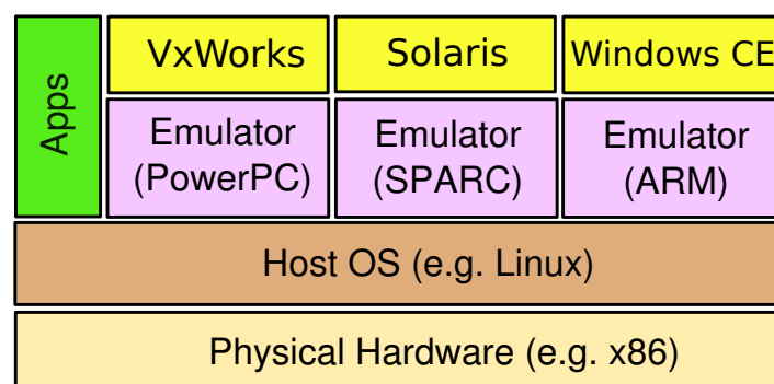
Figure 2.2: Emulation example
