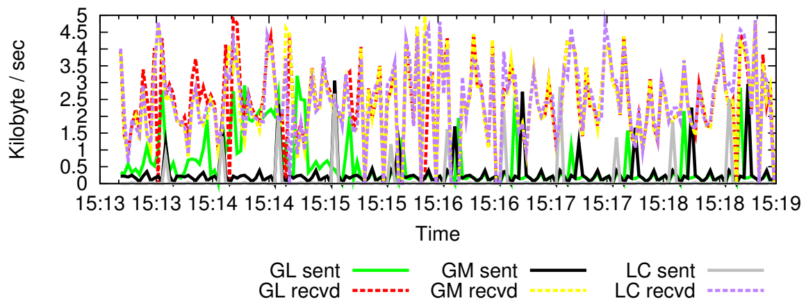
Figure 3.7: Snooze network load scalability
