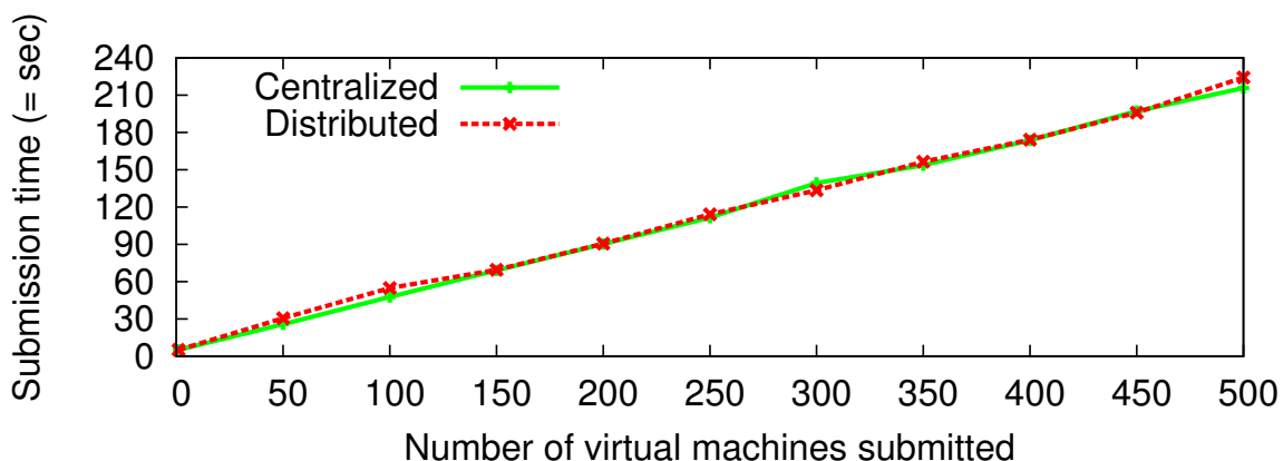
Figure 3.6: Snooze submission time: centralized vs. distributed
