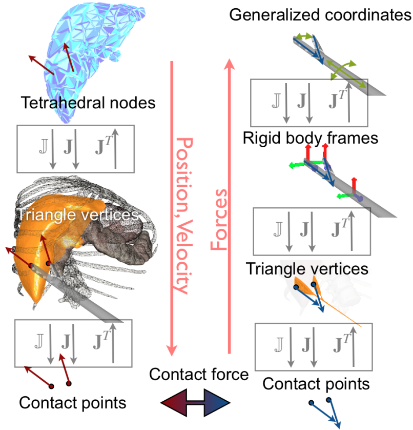
Figure 2.14: Mappings between the DOFs and the contact points. Left(top to bottom):the internal model of the liver is based on Finite Element model. A triangular mesh is mapped for collision detection with the surface. The two contact points found by the collision detection (with the grasper) are mapped on the collision model. Right (bottom to top): the contact points are also mapped on the collision model of the grasper. This collision model is a simplification of the grasper shape and is mapped on the rigid body frames. The motion of these frame is mapped on the state of the joints which are the independent DOFs of the grasper.
