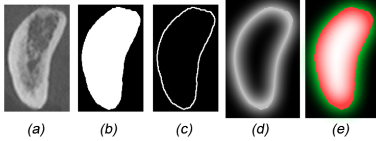
Figure 3.2: Illustration of 3D distance map extraction from CT-scan datas (here for one slice): (a) Original CT-scan slice (b) Binarization (c) Border extraction (d) 3D distance map to surface (e) Signed 3D distance map to surface (green = outside, positive, and red = inside, negative)
