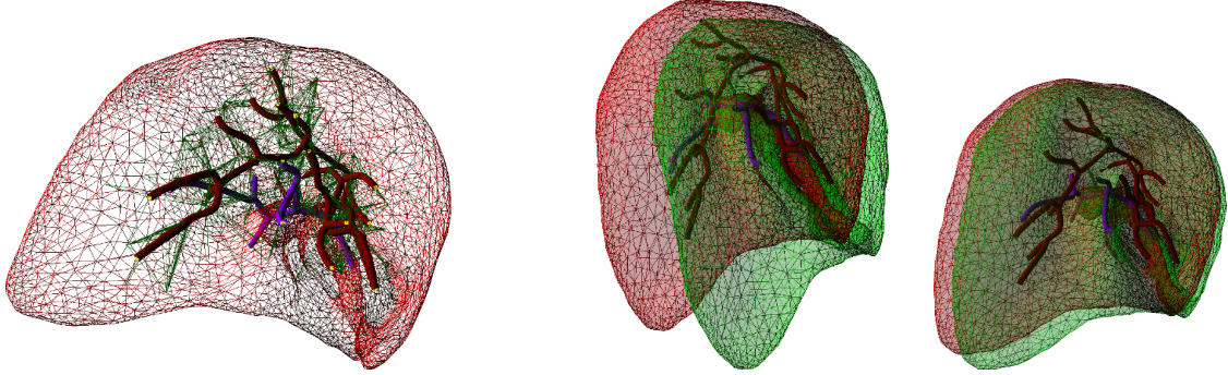
Figure 1.26: Vascularized model of liver: (a) initial position with mapped vascular trees, (b)(c) deformation of liver (stiffness 3500 kPa and 15000 kPa, respectively) under gravity (green: non-vascularized model, red: vascularized model)
