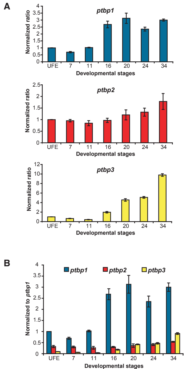
Fig. 2. Temporal expression profiles of polypyrimidine tract binding protein (PTB) genes during Xenopus development. (A) mRNA expression profiles normalized to the endogenous odc mRNA of each embryonic stage. Results are expressed with the normalized expression of the gene of interest in the Unfertilized Eggs (UFE) arbitrarily set to 1. (B) mRNA expression profiles normalized to ptbp1 mRNA. The amount of ptbp2 and ptbp3 mRNAs presented in (A) were normalized to that of ptbp1 transcripts in UFE arbitrarily set to 1. (A,B) The horizontal axes represent the UFE and embryos at the different developmental stages determined according to Nieuwkoop and Faber (Nieuwkoop and Faber, 1956).
