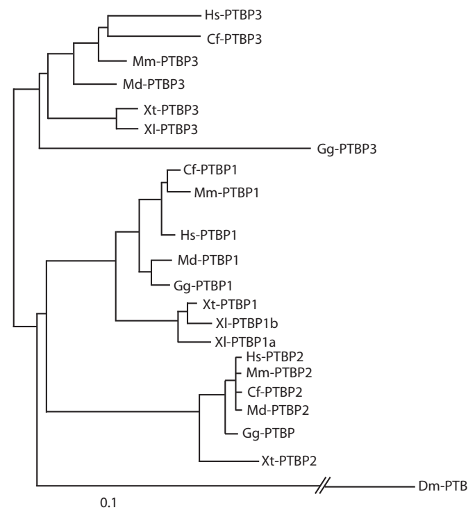
Fig. 1. Phylogenetic analysis of polypyrimidine tract binding protein (PTB) family members. The phylogenetic tree was constructed with the Neighbor-Joining method as described in the material and methods section. Parallel slanted lines designate interruptions of the normal scale and correspond to a distance of 0.5. The scale bar represents the number of amino acids substitutions. The abbreviations used are Cf: Canis familiaris, Dm: Drosophila Melanogaster , Gg: Gallus gallus ; Hs, Homo sapiens ; Md, Monodelphis domestica ; Mm, Mouse musculus ; Xi, Xenopus laevis ; Xt, Xenopus tropicalis .
