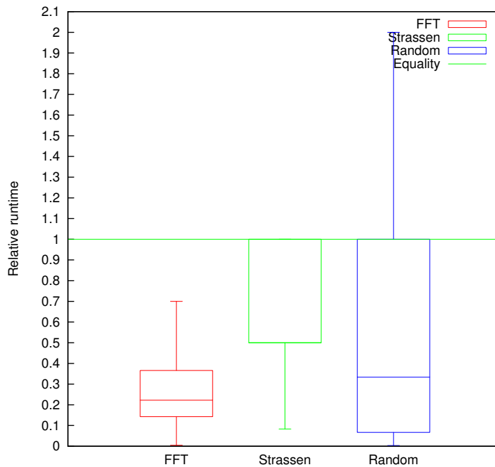
Figure 5.10: Relative runtime of the two allocation algorithms ( \frac{\text{Time to compute Eager}}{\text{Time to compute Deferred}} )
