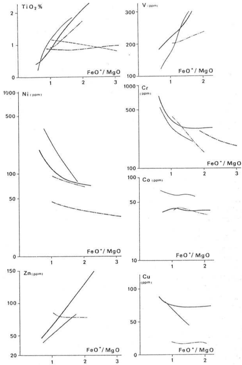
Fig. 1. Variation of the transition elements vs. the FeO^*/MgO ratio in some representative metabasic rocks suites. Amphibolites: Acebuches (Dupuy et al., 1979) (—); and Odenwald (Klemm and Weber-Diefenbach, 1971) (-.-). Granulites: Bournac (Leyreloup et al., 1977) (-.-.-); and Madras (Sen and Ray, 1971) (---). Eclogites: Hohen Tauern (Richter, 1973) (—). Shaded area: abyssal tholeiite fields after Andriambololona (1978).
