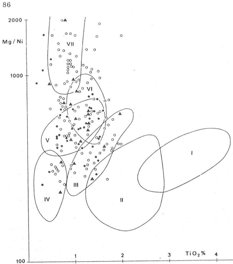
Fig. 3. Mg/Ni ratio vs. TiO 2 . Open circles : amphibolites (Van de Kamp, 1969; Prato, 1970; Klemm and Weber-Diefenbach, 1971; Knauer et al., 1974; Rivalenti and Rossi, 1975; Weber-Diefenbach, 1976; Dupuy et al., 1979; unpublished data for Rouergue, French Massif Central: C. Nicollet (1978); and Strona Valley: D.R. Andriambololona (1978). Triangles = granulites (Leyreloup et al., 1977; unpublished data for French Massif Central: Marchand; and Strona Valley: Andriambololona (1978). Full circles = eclogites (Bryhni et al. 1969; Ernst, 1977; Matthes and Seidel, 1977; Miller, 1970; Råheim, 1976; Richter, 1973; unpublished data for Rouergue: Nicollet (1978). Continuous lines define the fields occupied by alkali and transitional basalt (I); extrusive continental tholeiites (II); olivine abyssal tholeiites and oceanic island tholeiites (III); oceanic gabbros and olivine normative dolerites (IV); plagioclase abyssal tholeiites, quartz-normative dolerites and Skaergaard gabbro (Wager and Mitchell, 1951 (V); continental margin calc-alkali rocks (VI); and island arc tholeiites and calc-alkali rocks (VII).
