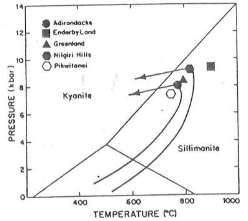
B : — P - T -time path for granulites consistent with magmatic heating of the lower crust before and during tectonic loading and initial, nearly isobaric cooling from peak conditions (symbols).
