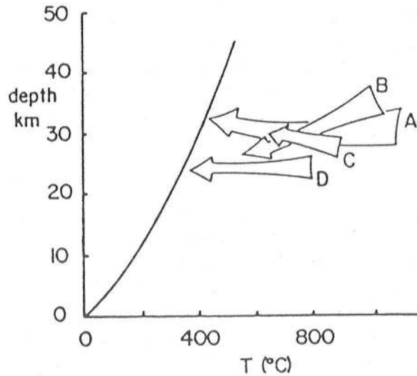
C : Cooling paths for (A) Basin and Range (hypothetical); (B) Enderby Land (Fyfe Hills) [29]; (C) Labwor Hills [21]; (D) Victorian lower crust
