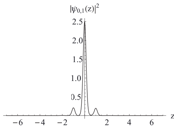
FIG. 2. Coordinate representation of the state |0,1\rangle belonging to the first Bloch band and centered in the zeroth well for U = 10 .
