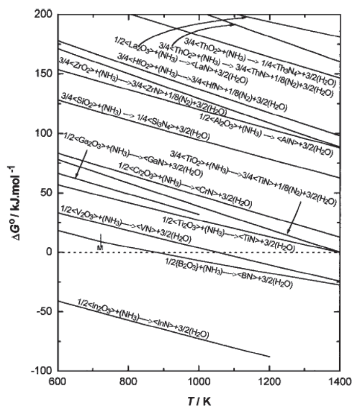
Figure I-6. Ellingham-Richardson-Jeffes diagram showing free standard enthalpy variation with temperature for the formation of nitrides from metallic oxides and ammonia. [73]
