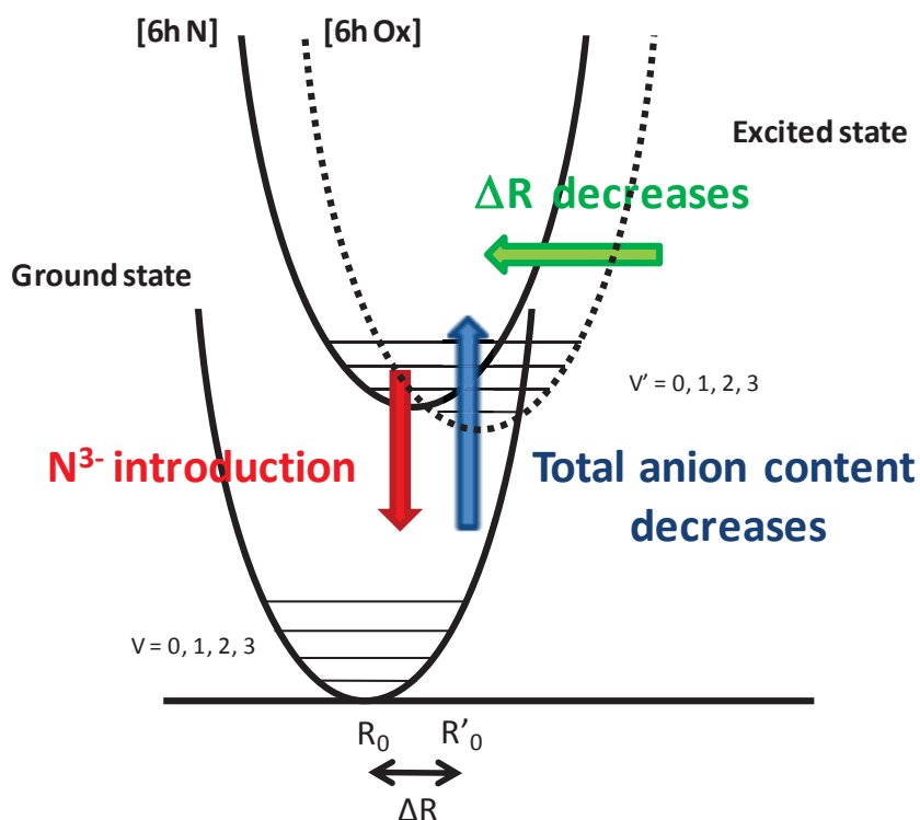
Figure III-19. Scheme for interpretation of the evolution of \text{Ce}^{3+} luminescence between 6h oxide (dashed line for excited state) and nitrided site (straight line for excited state).
