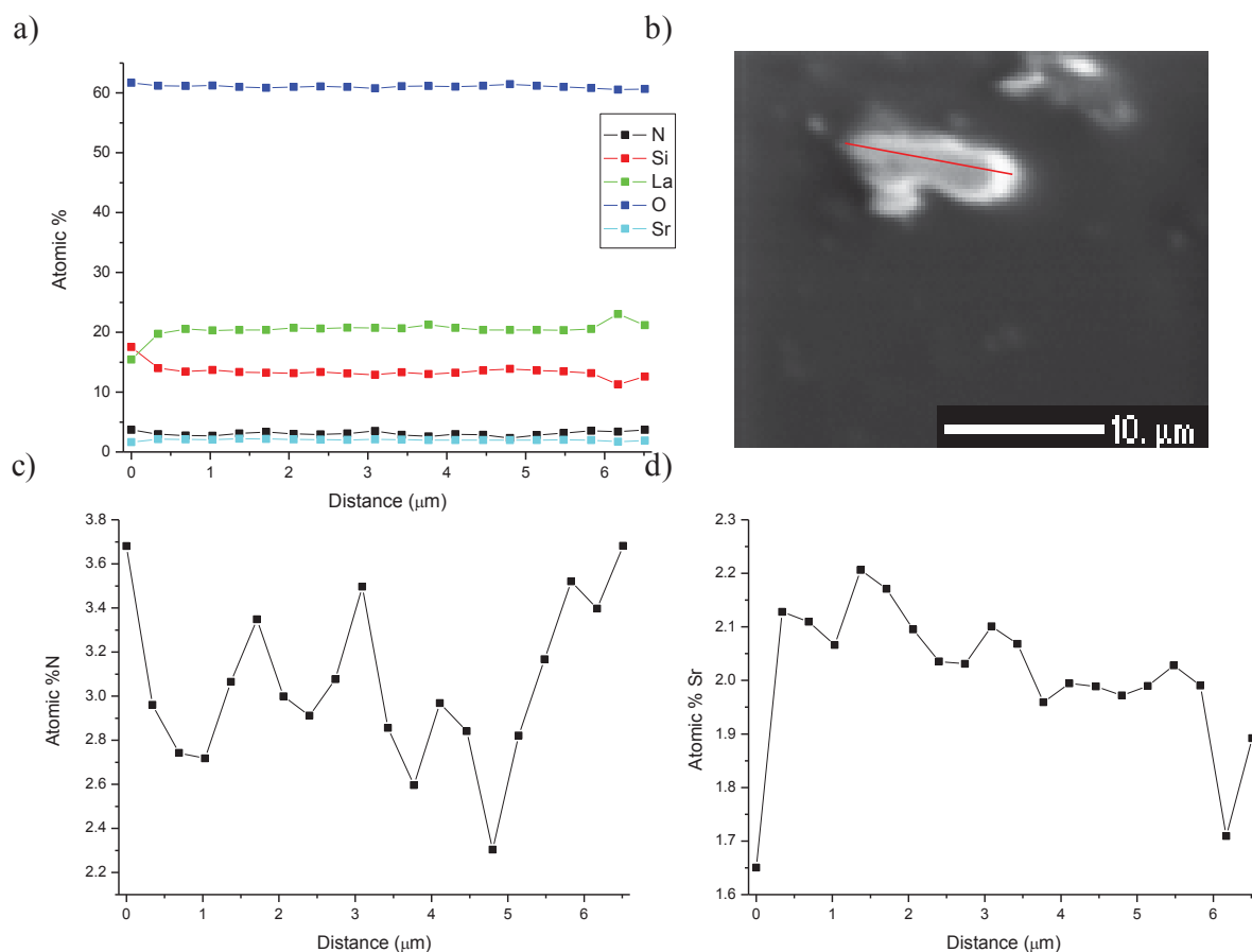
Figure II-20. Evolution of atomic % within the particle. a) All elements b) SEM picture of the particle with the chosen line in red c) Focus on N distribution d) Focus on Sr distribution.
