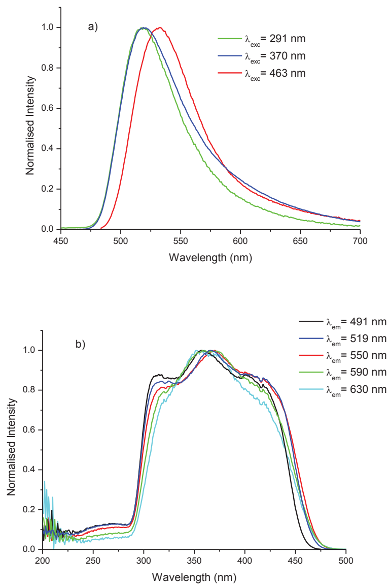
Figure III-10. Emission a) and excitation b) spectra at 4.2K of \text{La}_{8.67}\text{Sr}_{0.9}\text{Eu}_{0.1}\text{Si}_6\text{O}_{26} reduced under Ar/ \text{H}_2 .
