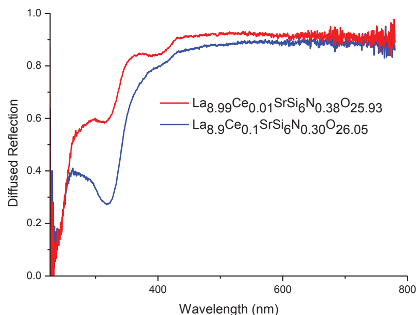
Figure III-21. Diffuse Reflection Spectra for two samples with different cerium concentrations
