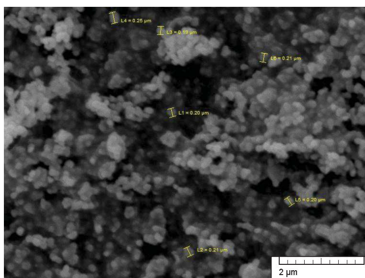
Figure II-5. Scanning electron microscopy image of \text{La}_{10}\text{Si}_6\text{O}_{25.23}\text{N}_{1.18} , prepared by ammonolysis of a sol-gel precursor.
