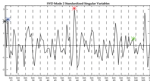
Figure IV.27: Expansion coefficient time series associated with each SST precursor ( left ) and projection of SST anomalies in JFM of each selected El Niño year onto the corresponding SVD mode ( right ), for (a) IOB, (b-c) SIO and (d) NPO precursor (see Table IV.3 for the spatial definition of these SST precursors).
