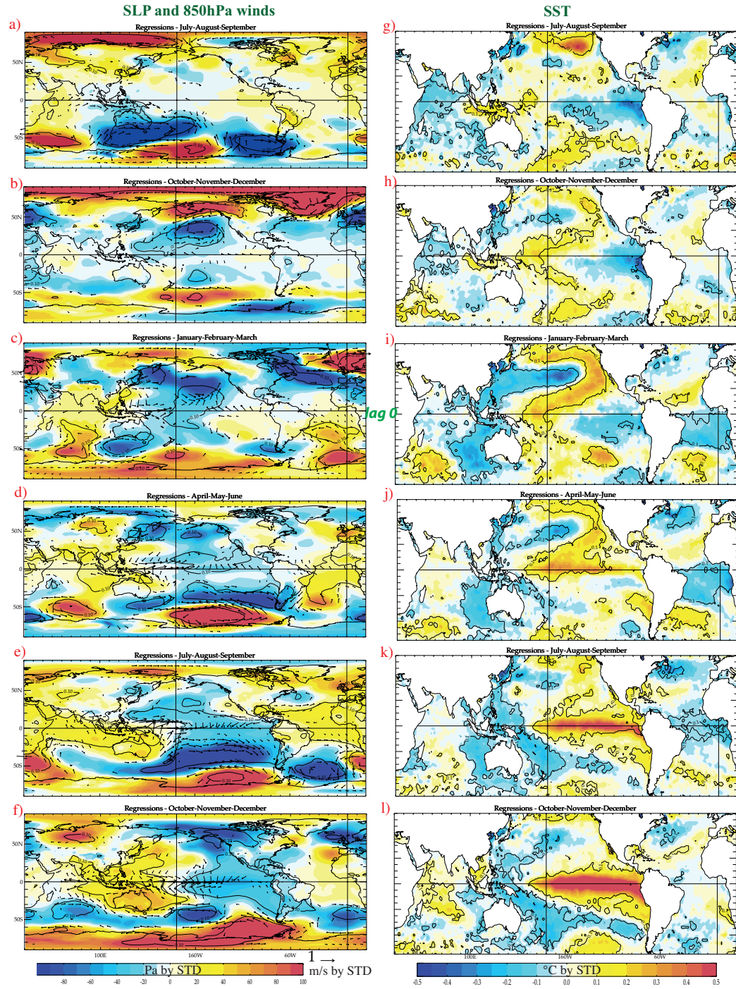
Figure 3 : SLP (shading) and 850hPa wind (vectors) anomalies (a to f) and SST anomalies (g to l) regressed onto the 2nd EOF time series of extratropical SST in JFM (over the 1979-2011 period). Maps are shown from the previous boreal summer to the following boreal winter. The black contours and the wind vectors denote that the corresponding correlation coefficients are above the 90% confidence level following a phase-scrambling procedure with 999 samples (Ebisuzaki, 1997).
