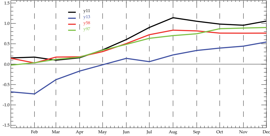
Figure IV.25: Projection of monthly SST anomalies in the tropical Pacific onto the SST singular vectors of the 1 st SVD(Z20-SST) mode (similar results obtained with the 1 st SVD(USTR-SST) mode), for each selected El Niño year.
