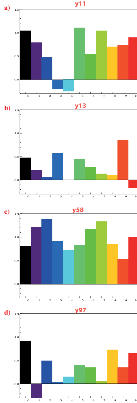
Figure IV.30: Projection of SST anomalies in the tropical Pacific during OND for a) y11, b) 13, c) 58 and d) y97 of the control run (black bar) and perturbed runs (coloured bars), onto the SST singular vectors of the 1 st of SVD (USTR-SST) mode.
