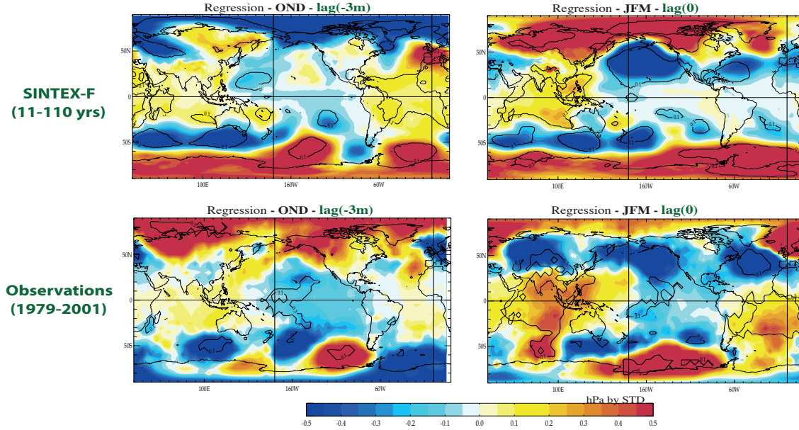
Figure IV.14: Lagged SLP anomalies regressed onto the SST expansion coefficient time series of the 1 st (a) and 2 nd (b) SVD mode between SIO SST in JFM and USTR anomalies in FMA, during the previous boreal fall in OND and synchronous JFM season, in the model ( top panels ) and observations ( bottom panels ).
