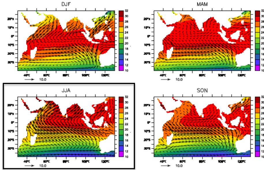
Figure I.3: SST and 10m wind climatological fields in the Indian Ocean, calculated from Hadley centre SST dataset [Rayner et al. , 2003] and from ERA40 reanalysis wind data [Uppala et al. , 2005] during the 1958-2001 period (from Manuel de météorologie tropicale : des alizés au cyclone , by Florent Beucher).
