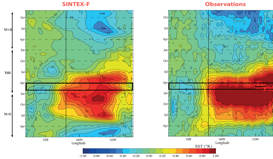
Figure IV.6: Time-Longitude Hovmöller plot of SST anomalies in the equatorial Pacific, regressed onto the USTR expansion coefficient time series of the 1 st (a) and 2 nd (b) SVD modes between (USTR-SST), from the previous to the following year, in the model ( left panels ) and in observations ( right panels ). The black box in these plots represents the 0 lag between SST anomalies and the zonal wind stress pattern (in FMA, see Fig IV.5)
