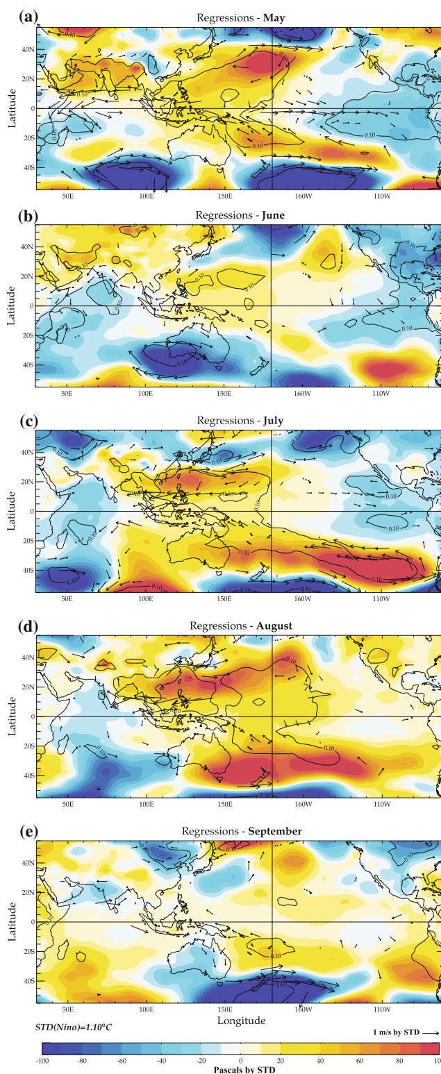
Fig. 5 Regression of \text{Nino}(-1) index onto monthly SLP (shading) and 850 hPa wind anomalies (arrows) from May to September. Regressions that are above the 90% confidence level estimated with a phase-scrambling bootstrap test with 999 sampled are encircled. Only wind anomalies that are above the 90% confidence level are shown. The standard deviation of the \text{Nino}3.4 index is given at the bottom of the panels
