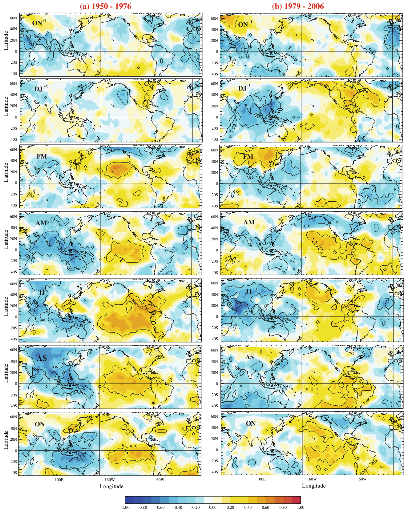
Fig. 4 Global correlation between ISM rainfall in JJ and bimonthly SLP anomalies from the boreal fall preceding ( \text{ON}^{-1} ) to that following (ON) the ISM season during a 1950–1976 and
