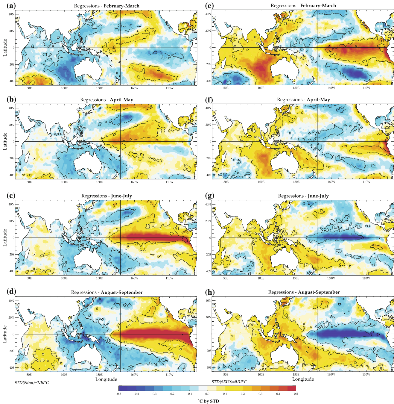
Fig. 9 Bimonthly SST anomalies regressed onto the Nino(0) index (a–d) and SEIO index (e–h) from February–March (FM) to August–September (AS). Regressions that are above the 90% confidence level
