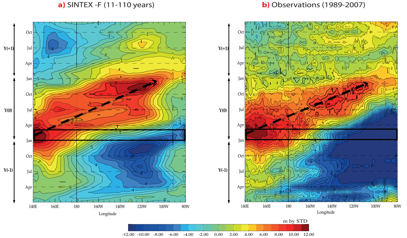
Figure IV.4: Time-Longitude Hovmöller plot of 20^{\circ}\text{C} isotherm depth (Z20) anomalies in the equatorial Pacific, regressed onto the Z20 expansion coefficient time series of the 1 st SVD mode between (Z20-SST), from the previous to the following year, in the model (a) and in observations (b).
