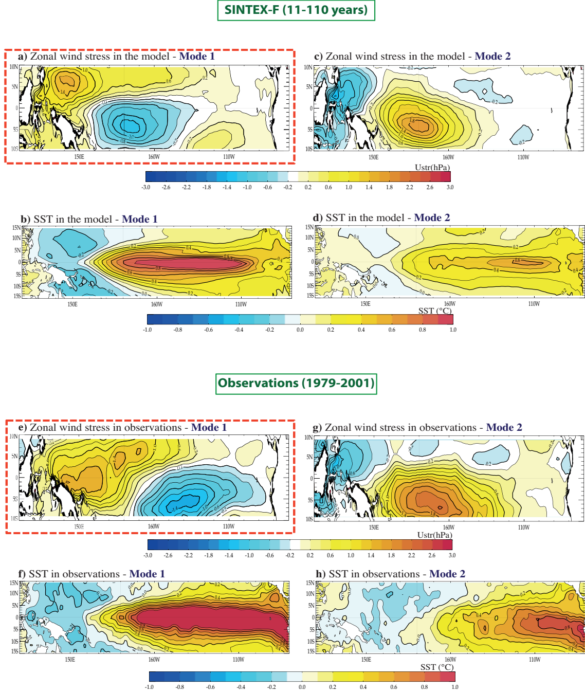
Figure IV.5: Zonal Wind Stress (USTR) and SST homogeneous maps associated with the 1 st (left panels) and 2 nd (right panels) SVD modes between USTR anomalies in FMA and SST anomalies in ONDJF in the tropical Pacific Ocean ([110°E-70°W,10°S-10°N] for USTR and [120°E-80°W,15°S-15°N] for SST), separately in the model (a-d) and in observations (e-h).
