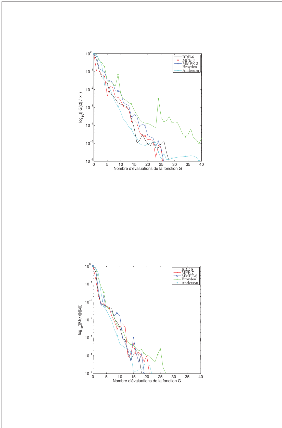
FIGURE 4.10 – Atome C, méthodes cycliques, \omega = 0.1, 0.2
