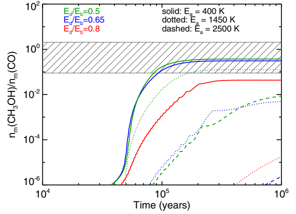
Fig. 10. Mantle CH 3 OH/CO abundance ratio versus time. The blue, green, and red lines refer to E_d/E_b = 0.65, 0.5, and 0.8, respectively. Solid, dotted, and dashed lines refer to E_a = 400 \text{ K}, 1450 \text{ K}, and 2500 \text{ K}, respectively. In these computations the density is 10^5 \text{ cm}^{-3} . The box with hatching shows the interval of CH 3 OH/CO abundance ratio observed towards intermediate- and high- mass protostars (Table 5). Because low-mass protostars provide only less stringent upper limits, they are not reported in the plot.
