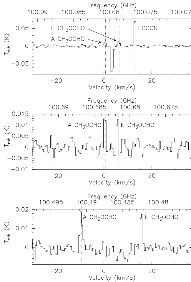
Figure 10.2: \text{CH}_3\text{OCHO} spectra of the 9_{17} - 7_{11} transitions at 100.48 GHz (A and E substates, bottom panel), of the 9_{09} - 8_{08} transitions at 100.68 GHz (A and E substates, middle panel), and of the 9_{19} - 8_{18} transitions at 100.08 GHz (A and E substates, top panel) in L1689B. The vertical dotted lines indicate the rest frequencies measured in the laboratory and listed in the JPL database. The \text{CH}_3\text{OCHO} spectrum in the top panel also shows a \text{HC}_3\text{N} line. The negative spectral feature between both \text{CH}_3\text{OCHO} lines results from the frequency switching procedure and the folding of the ortho- \text{CH}_2\text{CO} line shown in Fig. 10.4.
