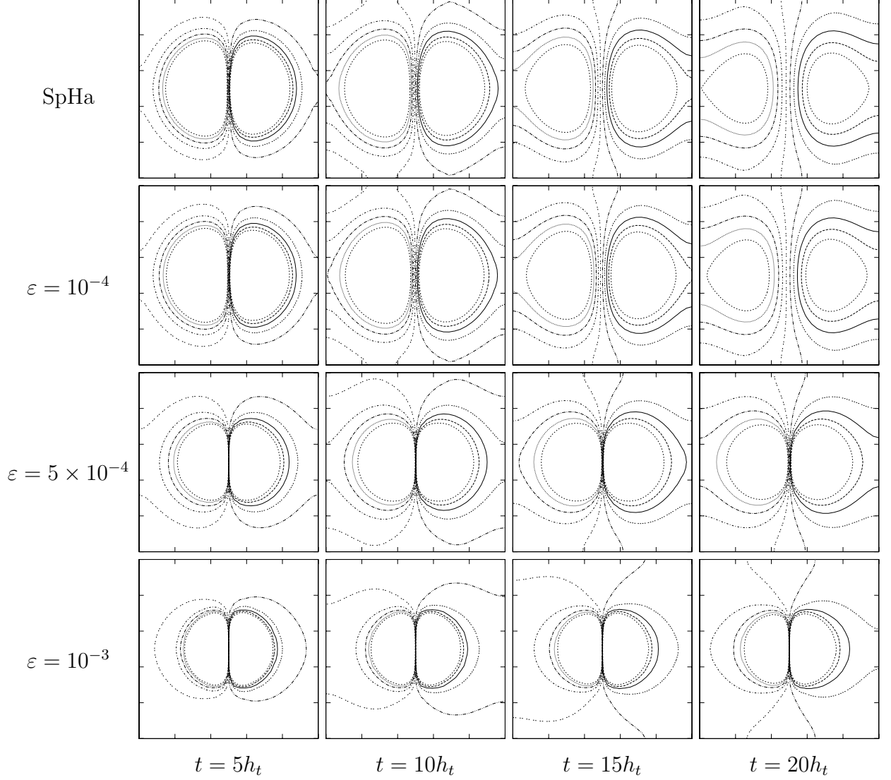
Figure IV.6: Temperature isoline (from 1.491 to 1.509 every 2 \times 10^{-3} ) with (2.11) (first line) and for several value of \varepsilon with (2.15) at some time iterations.
