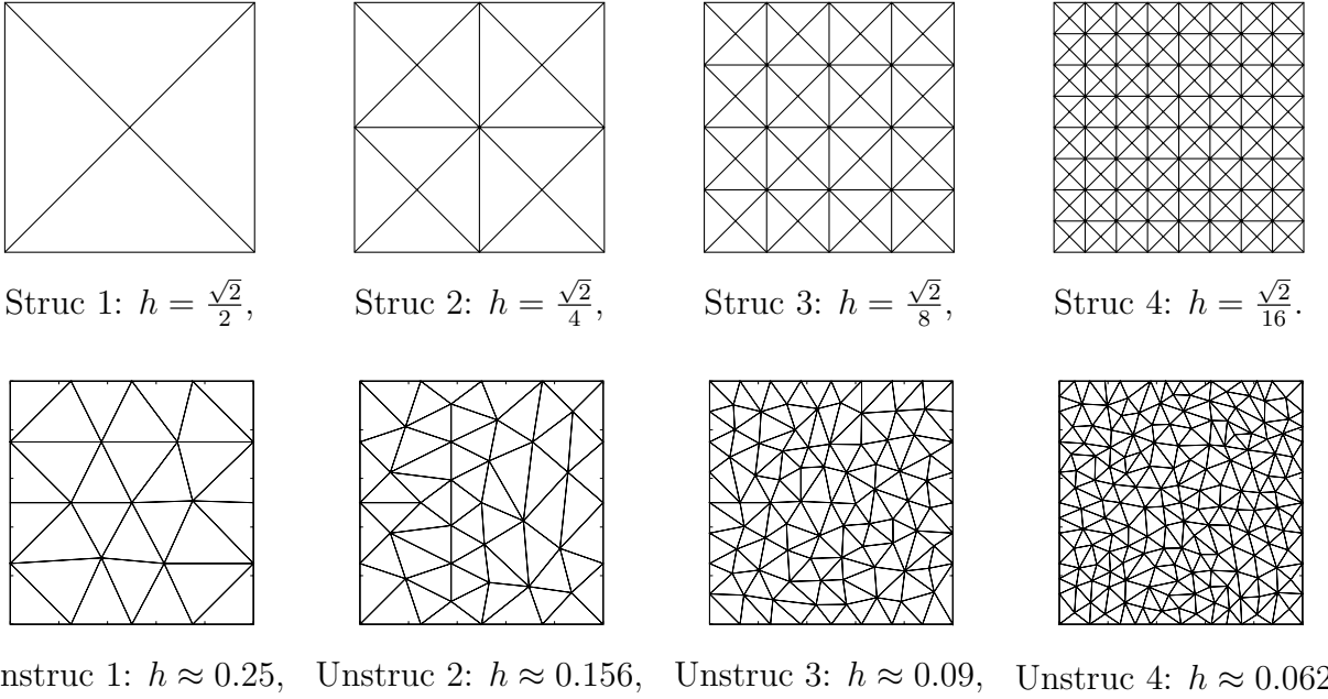
Figure IV.3: Examples of mesh used to estimate the consistence. In the first line, structured meshes obtained with iterative process, Struc n is the union of four Struc n - 1 scaled by 1/2 . In the second line, unstructured meshes obtained by Delaunay triangulation using the mesh generator Triangle .
