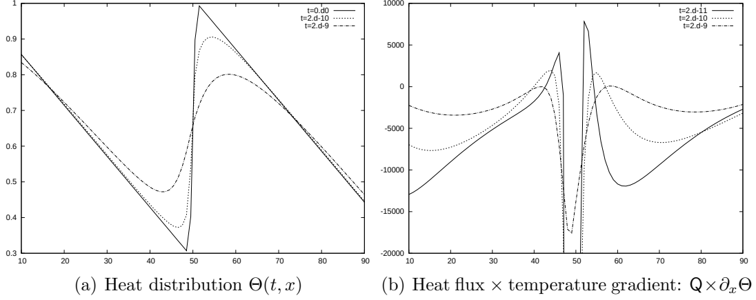
Figure II.2: Kinetic results: Simulation of a kinetic model ( fpelec code from CEA)
