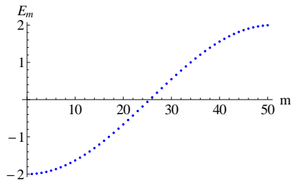
Figure A.1: Eigenvalues of 1D chain. The size is chosen N=50 sites and the parameters \epsilon = 0 and t = 1 . All the eigenvalues are non degenerate
