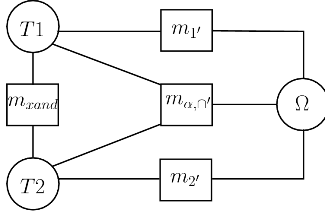
Figure 6.2: Valuation network for the \alpha -conjunction of two BBAs m_1 and m_2 . In the network, the term (\odot_{x \in \Omega} m^{T_1 \times T_2}[x] \uparrow^{\Omega \times T_1 \times T_2}) appearing in Theorem 6.1, is replaced by a BBA m_{\alpha, \cap'} defined on \Omega \times T_1 \times T_2 .
