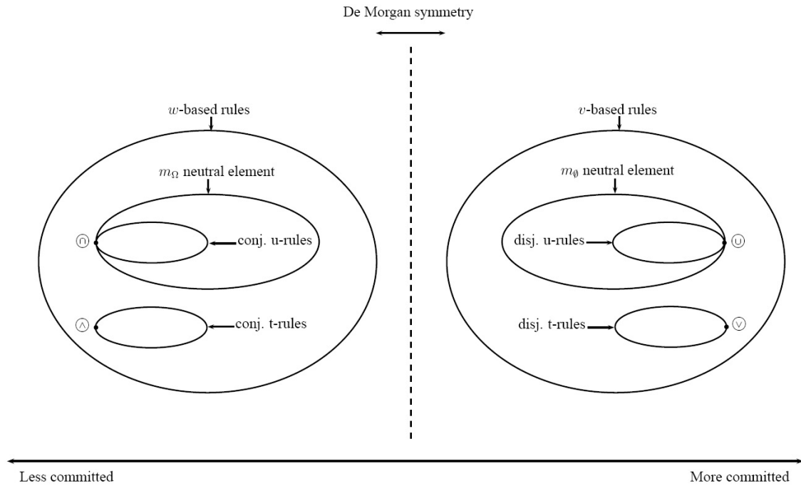
Figure 4.4: The four families of combination rules studied in this chapter, and the singular positions of the four basic rules \oplus , \wedge , \odot and \vee .
