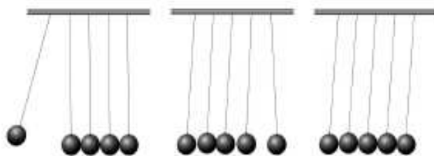
Figure 3.7. Three Phase of Newton's Cradle dynamics: (1) 'end bounce', (2) 'middle jostle', and (3) 'joint swing'. Source: Lowe (2006)
