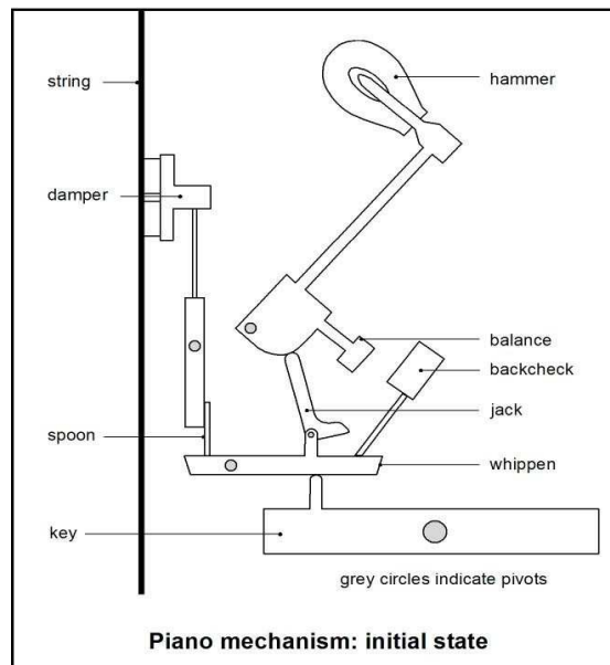
Figure 7.1. An upright piano mechanism (Boucheix and Lowe, 2008)
