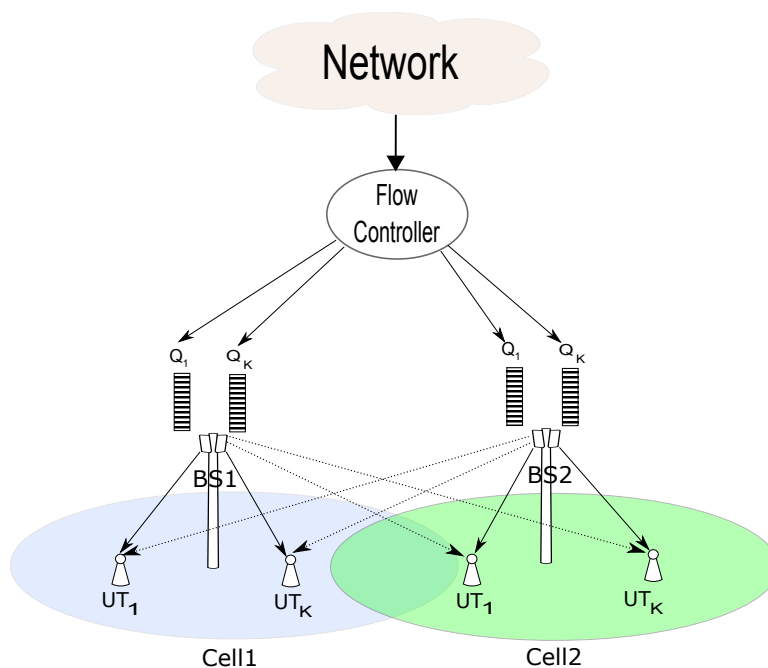
Figure 3.1: System Setup
