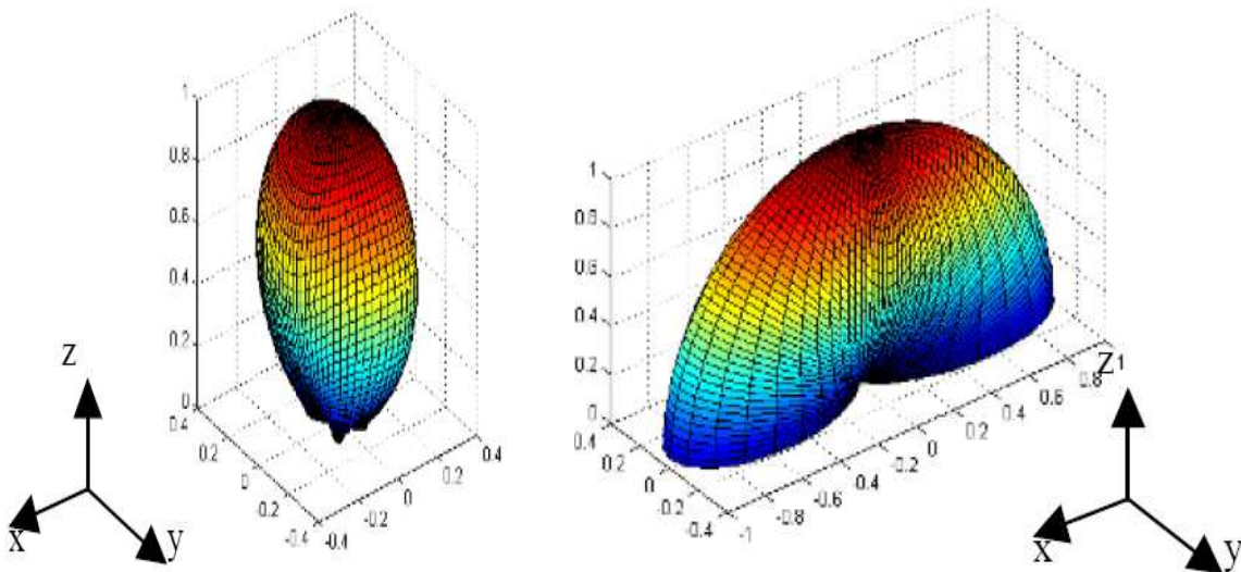
Fig2.23: E-plane and H-plane arrays arranged along x-axis and y-axis [2]
