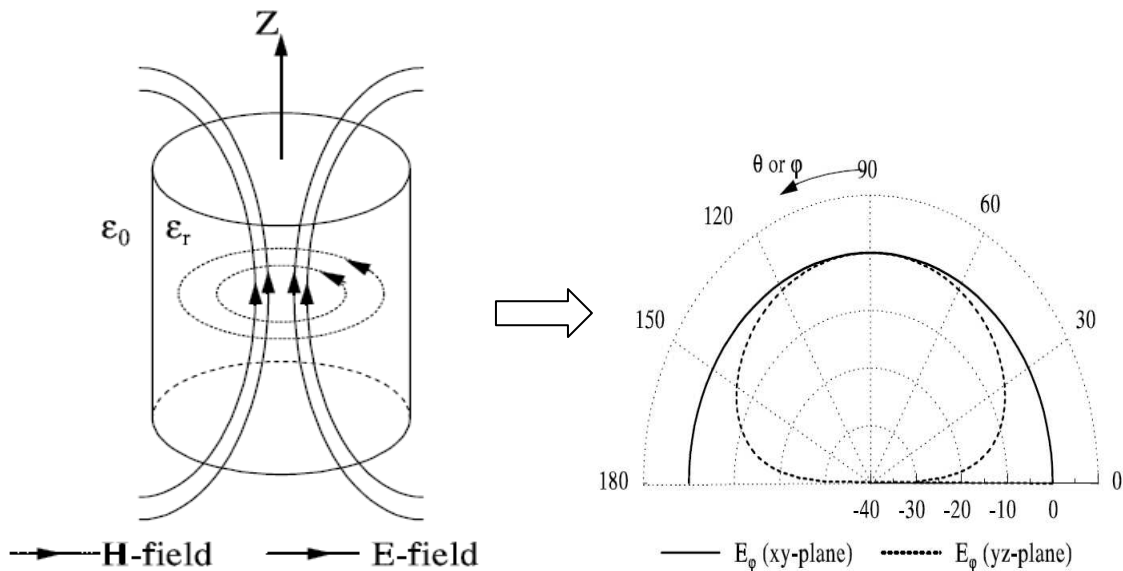
Fig2.8: Mode TE_{01} and its broadside far field radiation pattern [1].
