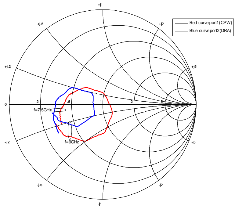
Fig3.40: X band DRA Port1 and Port2 Smith chart curves
