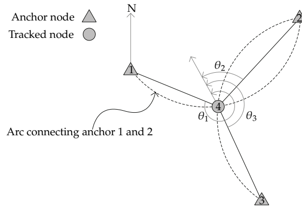
Figure 2.5: Location estimation using AoA
