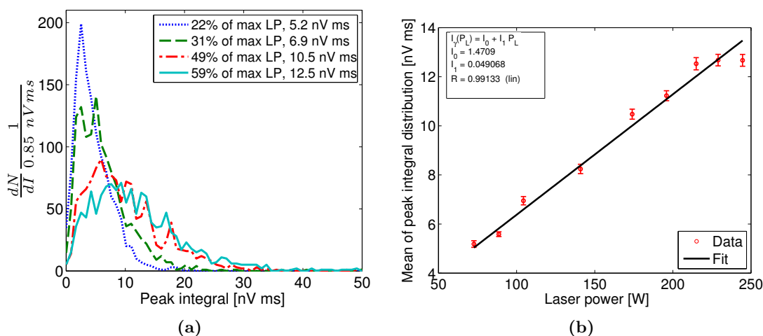
Figure 5.30: Gamma ray spectrum for different FPC stored laser power - Fig. 5.30a presents gamma ray spectrum for different FPC stored laser power. Different colors correspond to the spectra taken at different FPC powers. In the legend, the fraction of the maximum FPC stored power and the mean of each of these spectra are shown. Fig. 5.30b shows the linear relation between the mean of gamma spectra for each laser power bin and the correspondent laser power which is defined as a mean of the laser power bins shown on Fig. 5.28a. The errors bars indicate the statistical errors.
