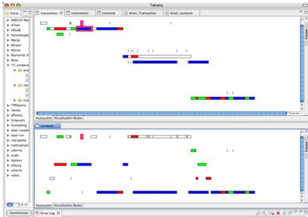
Figure 5-7 Two visualisations of the same corpus. Both visualisations distinguish participants by colour. In the top visualisation, the three major rows correspond with the three phases. Within each of these, the minor rows indicate which communication media was used.
