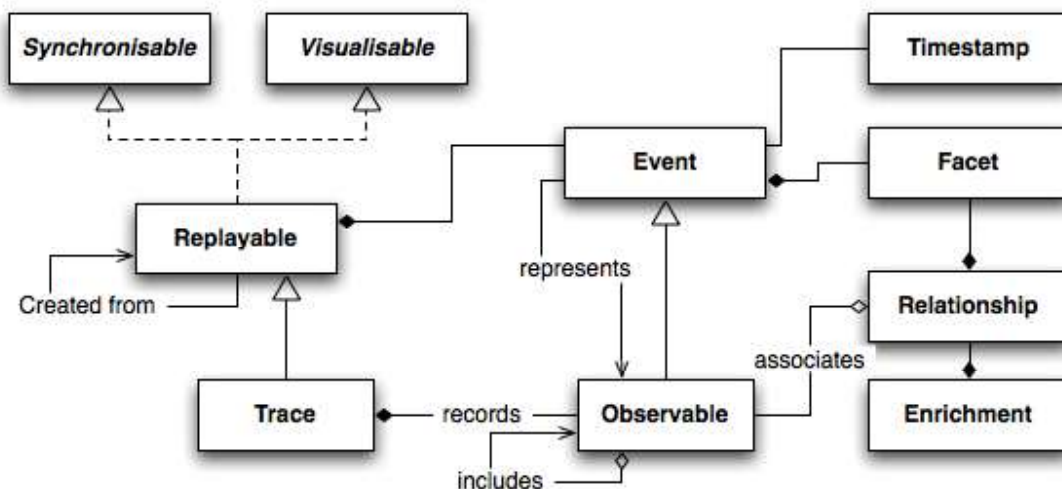
Figure 3-5 UML class diagram showing the main aspects of the proposed model for replayables.
