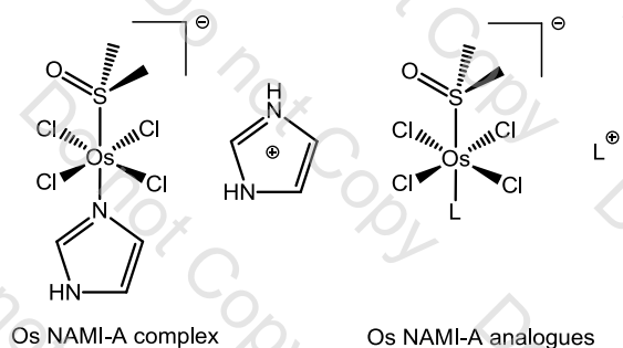
Figure 30: Anticancer osmium(III) Nami-A type analogues
