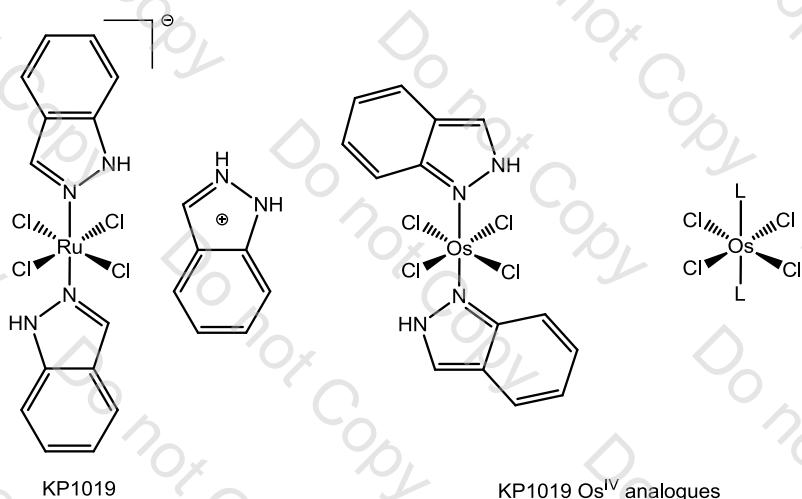
Figure 32: KP1019 and anticancer osmium(IV) analogues
