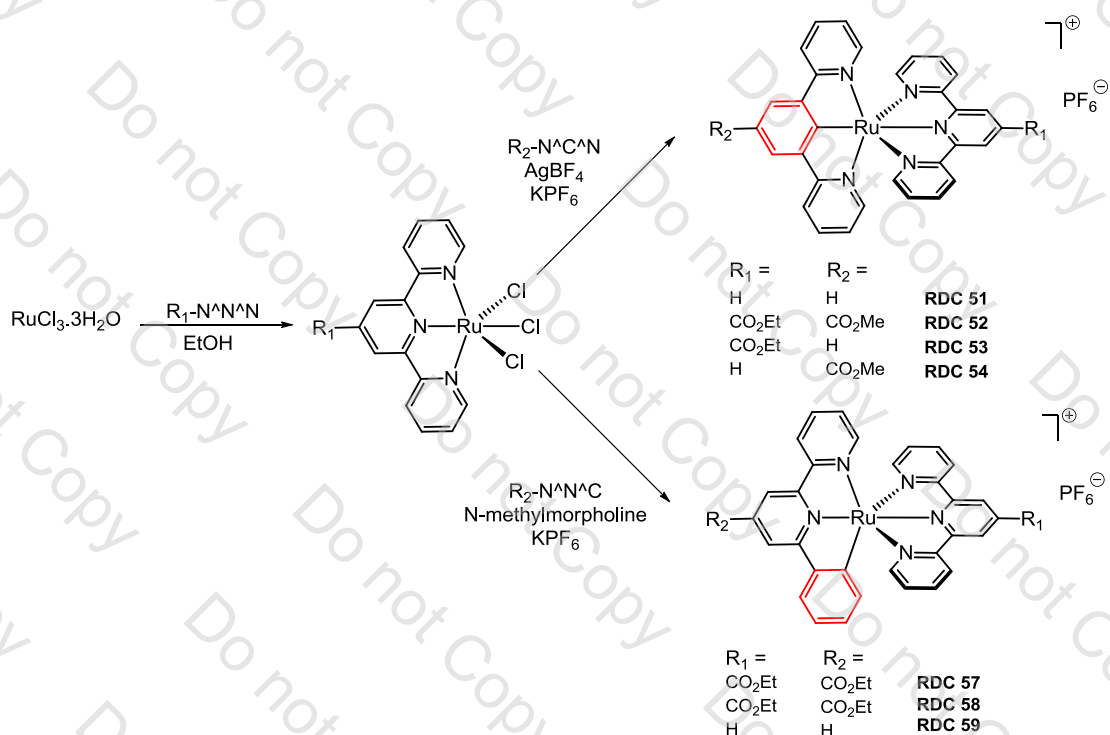
Figure 1: Synthesis of second generation RDCs containing N^{\wedge}C^{\wedge}N' or N^{\wedge}N^{\wedge}C pincers and substituted terpy ligand
