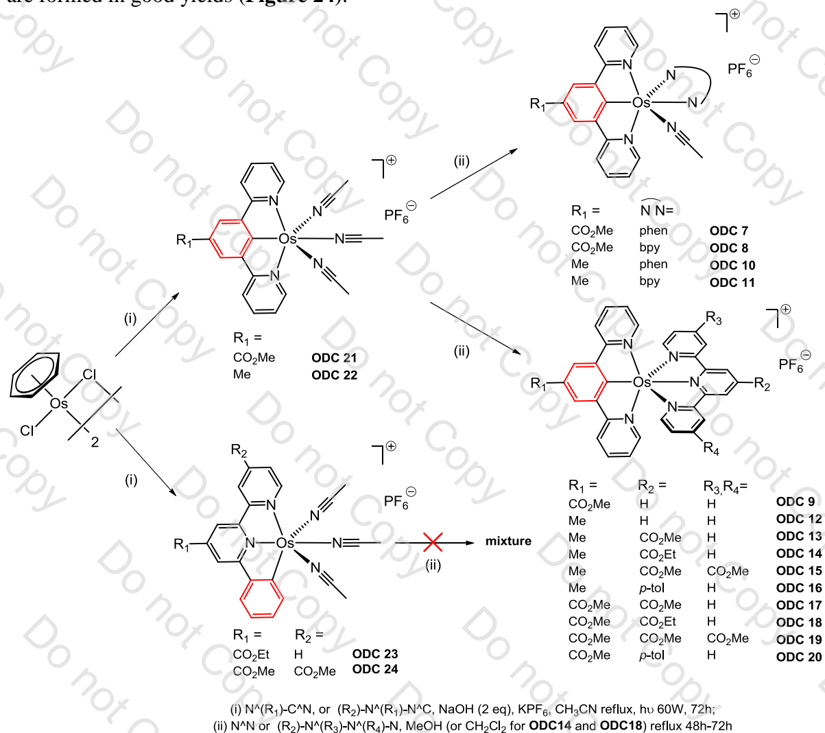
Figure 24: Synthesis of second generation ODCs containing N ^ C ^ N ^ or N ^ N ^ ^C pincers
