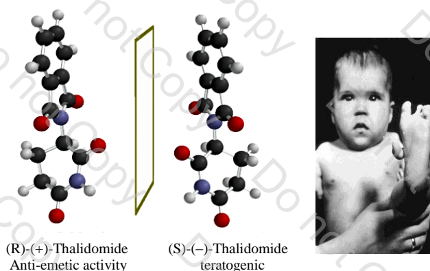
Figure 35: The two enantiomers of Thalidomide
