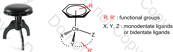
Figure 35: General structure of half-sandwich arene osmium complexes
