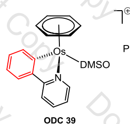
Figure 17: Impact of substitution of MeCN by DMSO on the antiproliferative activity (A172 glioblastoma cell line)
