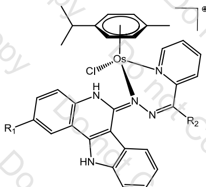
Figure 40: Chemical structure of indoloquinoline-type arene-osmium(II) complexes
