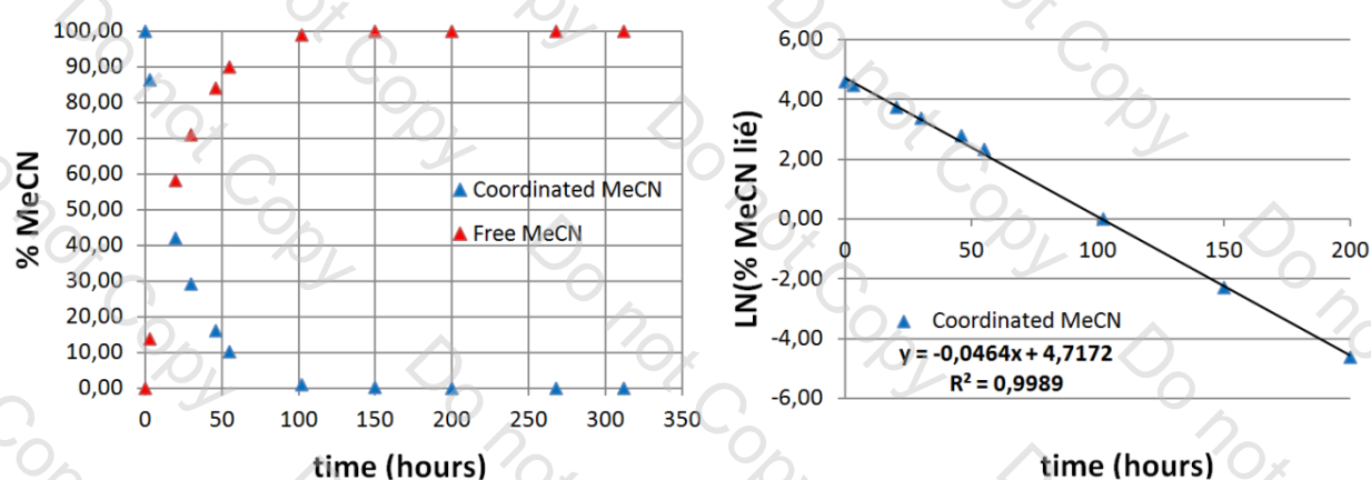
Figure 11: Evolution of ODC 4 in DMSO- d_6 monitored by ^1\text{H} NMR spectroscopy at R.T.
