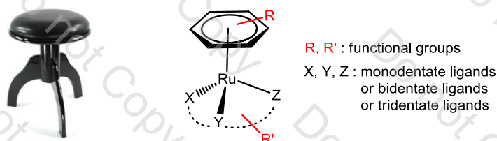
Figure 17: General structure of half-sandwich arene ruthenium complexes
