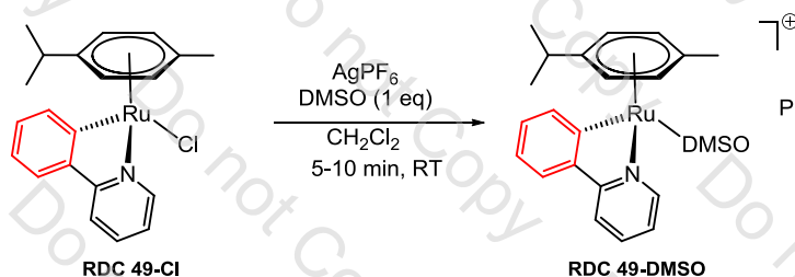
Figure 27: Synthesis of RDC 49-DMSO
