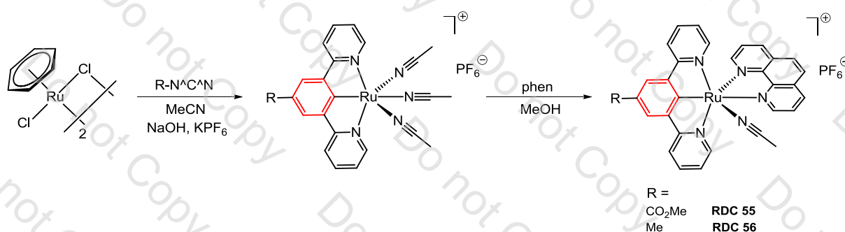
Figure 2: Synthesis of second generation RDCs containing \text{N}^{\wedge}\text{C}^{\wedge}\text{N} substituted pincers and bidentate 2,2'-phenanthroline
