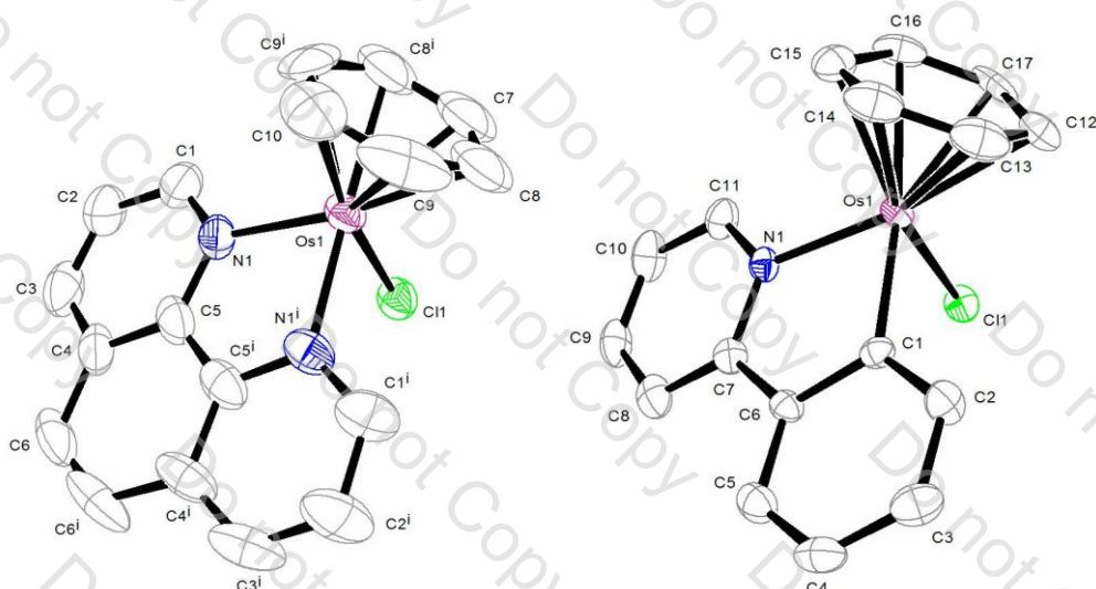
Figure 1: ORTEP diagram of the molecular structure of ODC 25 (left) and ODC 38 (right).
