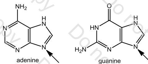
Figure 9: N7 nitrogen atom of adenine and guanine reacting with cisplatin
